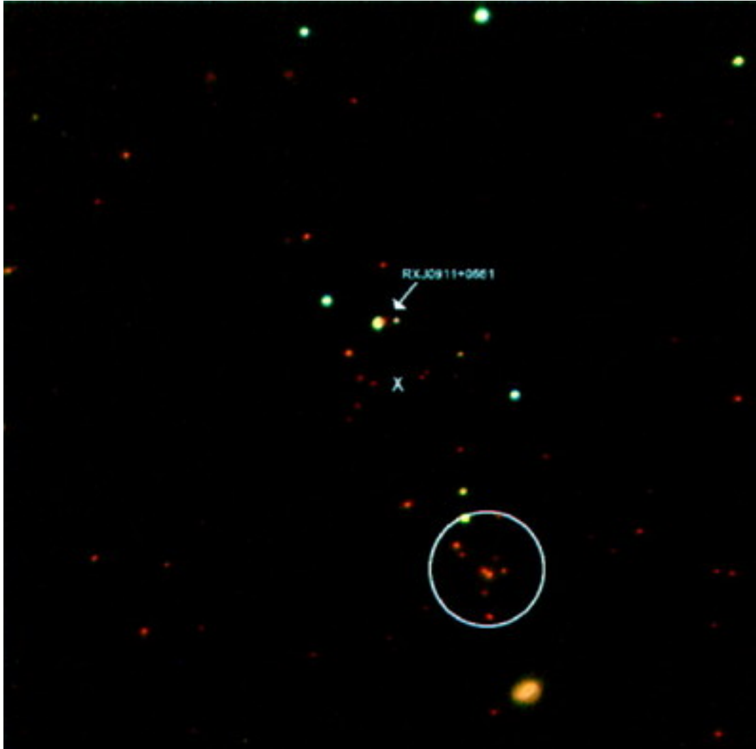
Fig. 2. from HighResolution Optical and NearInfrared Imaging of the Quadruple Quasar RX J0911.4+0551 Burud et al. 1998 ApJL 501 L5 doi:10.1086/311450 https://dx.doi.org/10.1086/311450 © 1998. The American Astronomical Society. All rights reserved. Printed in U.S.A.
