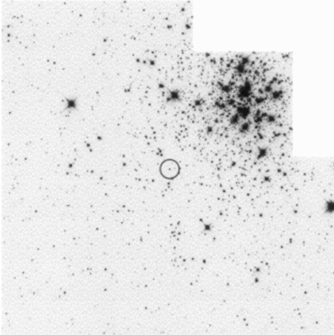
Fig. 2. from Discovery of a Luminous White Dwarf in a Young Star Cluster in the Large Magellanic Cloud Discovery of Luminous White Dwarf 1998 ApJL 499 L53 doi:10.1086/311349 https://dx.doi.org/10.1086/311349 © 1998. The American Astronomical Society. All rights reserved. Printed in U.S.A.
