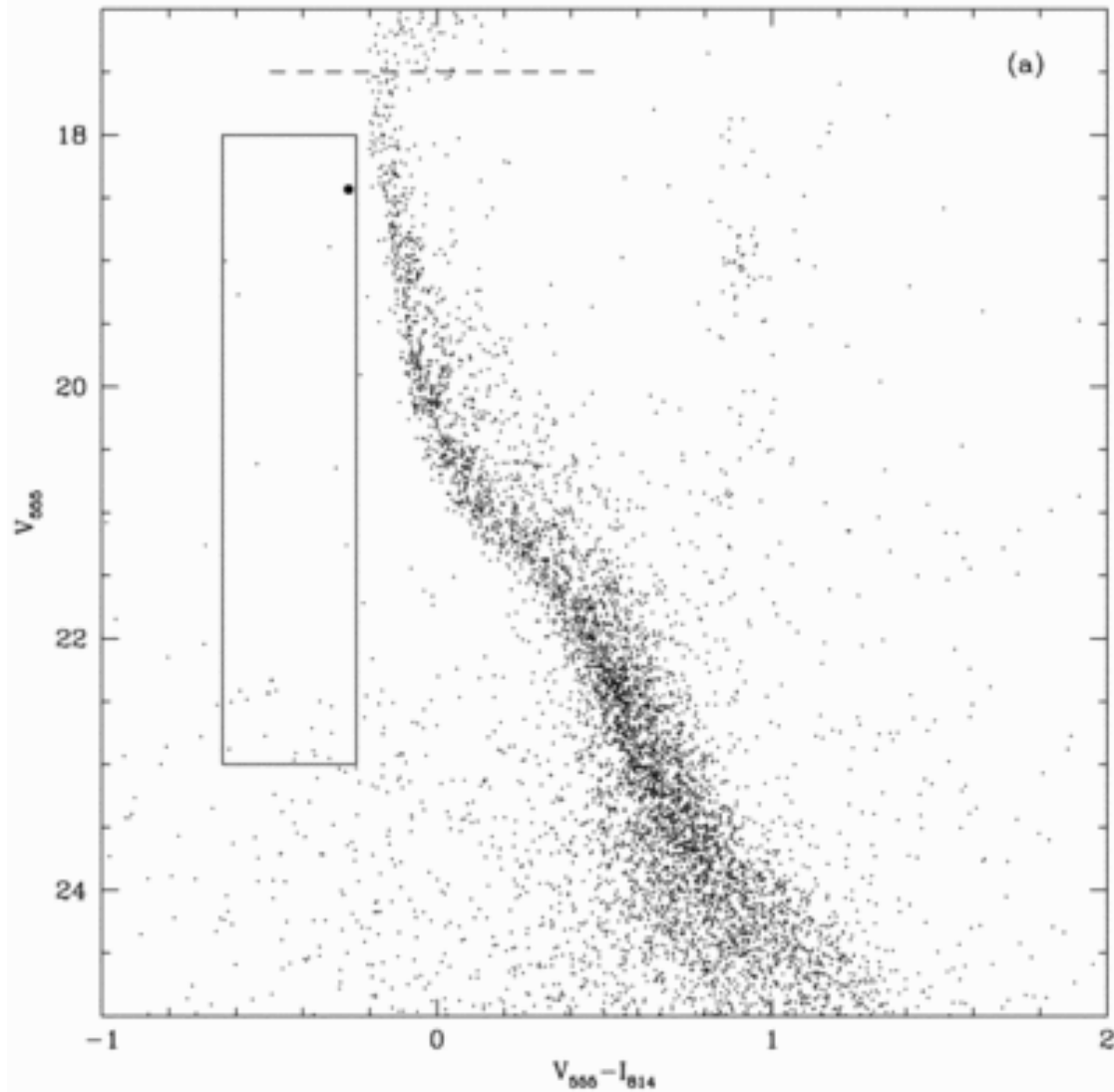
Fig. 1. from Discovery of a Luminous White Dwarf in a Young Star Cluster in the Large Magellanic Cloud Discovery of Luminous White Dwarf 1998 ApJL 499 L53 doi:10.1086/311349 https://dx.doi.org/10.1086/311349 © 1998. The American Astronomical Society. All rights reserved. Printed in U.S.A.
