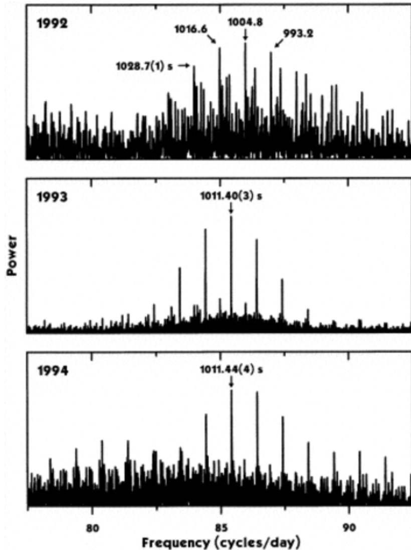
Fig. 2. from The Orbital Period of AM Canum Venaticorum Harvey et al. 1998 ApJL 493 L105 doi:10.1086/311143 https://dx.doi.org/10.1086/311143 © 1998. The American Astronomical Society. All rights reserved. Printed in U.S.A.
