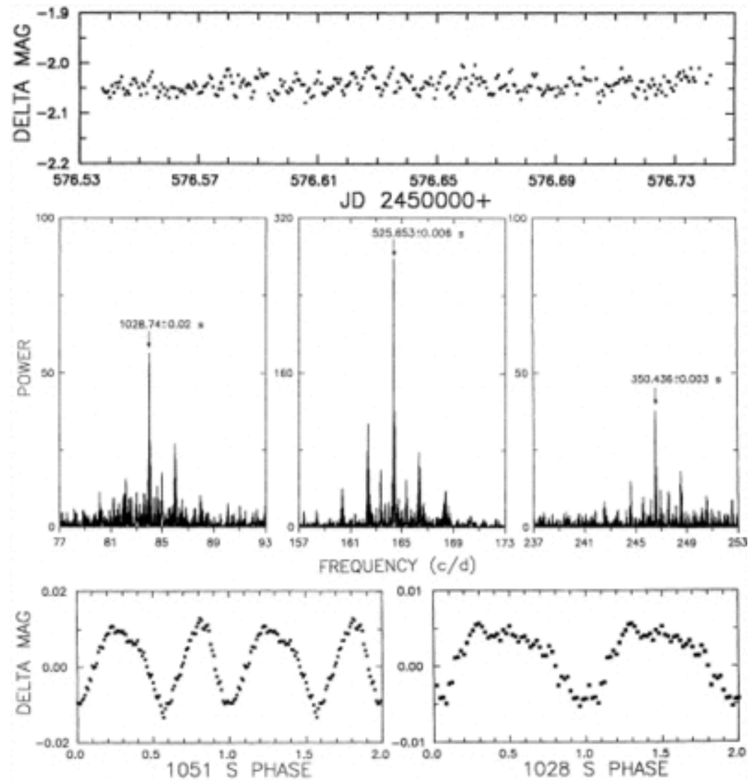
Fig. 1. from The Orbital Period of AM Canum Venaticorum Harvey et al. 1998 ApJL 493 L105 doi:10.1086/311143 https://dx.doi.org/10.1086/311143 © 1998. The American Astronomical Society. All rights reserved. Printed in U.S.A.
