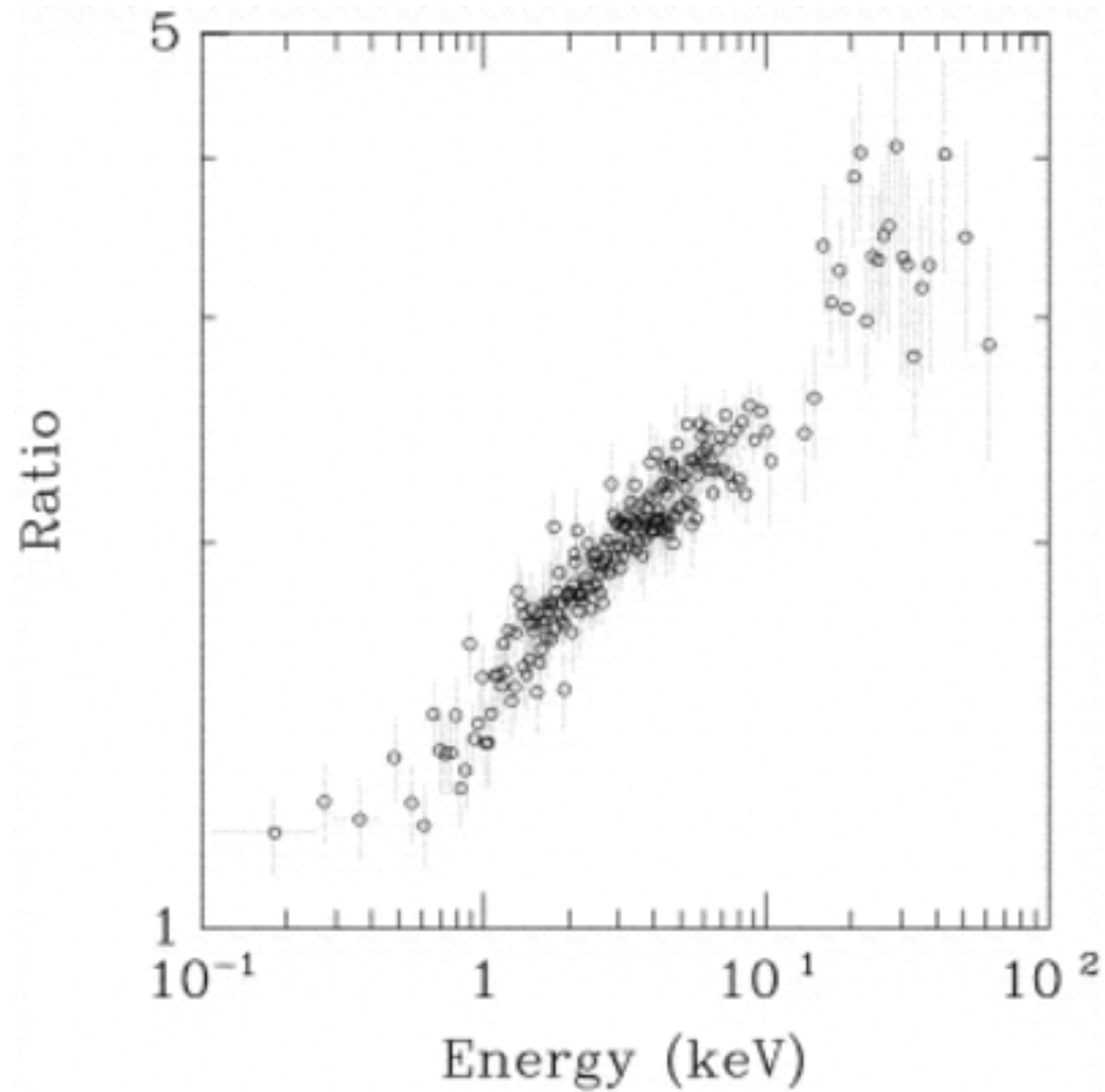
Fig. 2. from BeppoSAX Observations of Unprecedented Synchrotron Activity in the BL Lacertae Object Markarian 501 Pian et al. 1998 ApJL 492 L17 doi:10.1086/311083 https://dx.doi.org/10.1086/311083 © 1998. The American Astronomical Society. All rights reserved. Printed in U.S.A.
