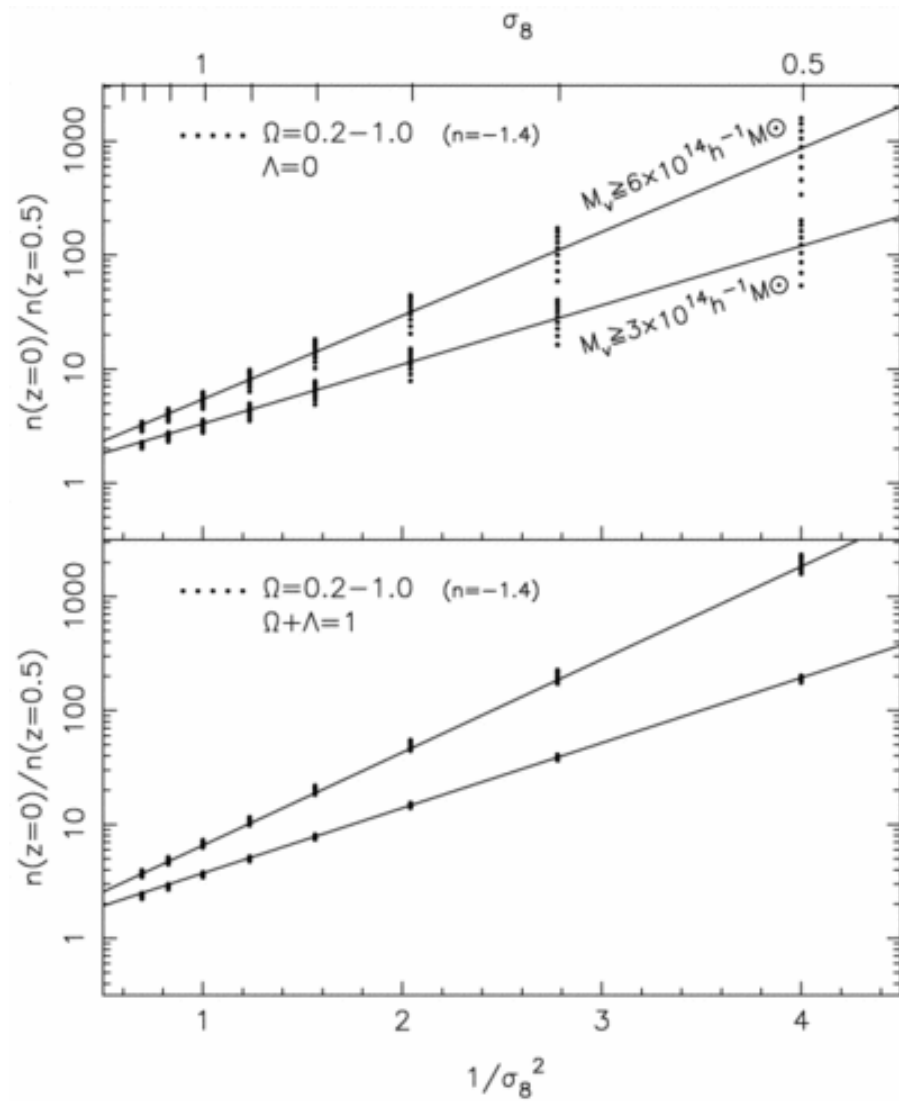
Fig. 3. from Determining the Amplitude of Mass Fluctuations in the Universe Fan, Bahcall, & Cen 1997 ApJL 490 L123 doi:10.1086/311031 https://dx.doi.org/10.1086/311031 © 1997. The American Astronomical Society. All rights reserved. Printed in U.S.A.
