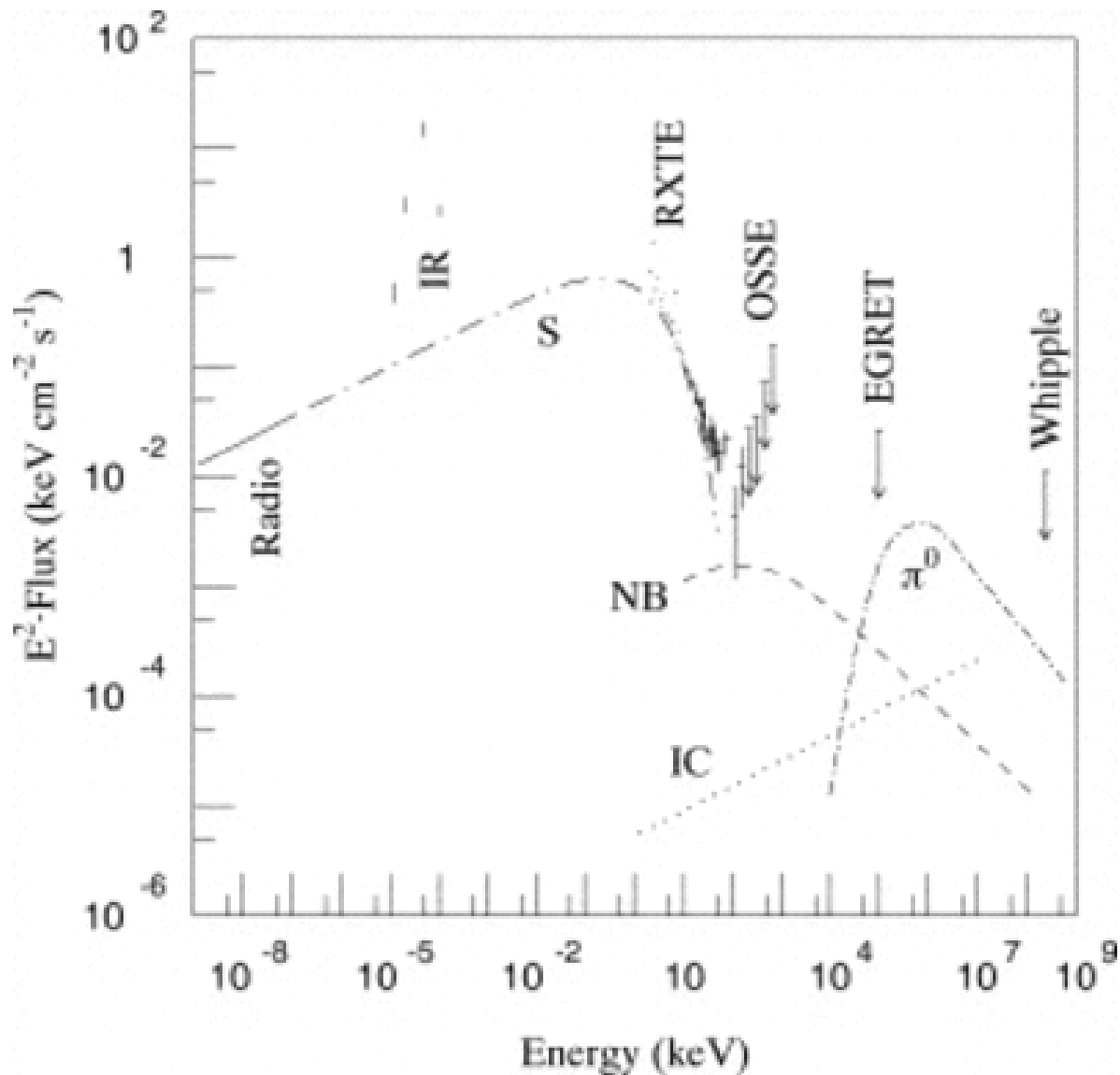
Fig. 3. from Evidence of XRay Synchrotron Emission from Electrons Accelerated to 40 TeV in the Supernova Remnant Cassiopeia A Allen et al. 1997 ApJL 487 L97 doi:10.1086/310878 https://dx.doi.org/10.1086/310878 ©1997. The American Astronomical Society. All rights reserved. Printed in U.S.A.
