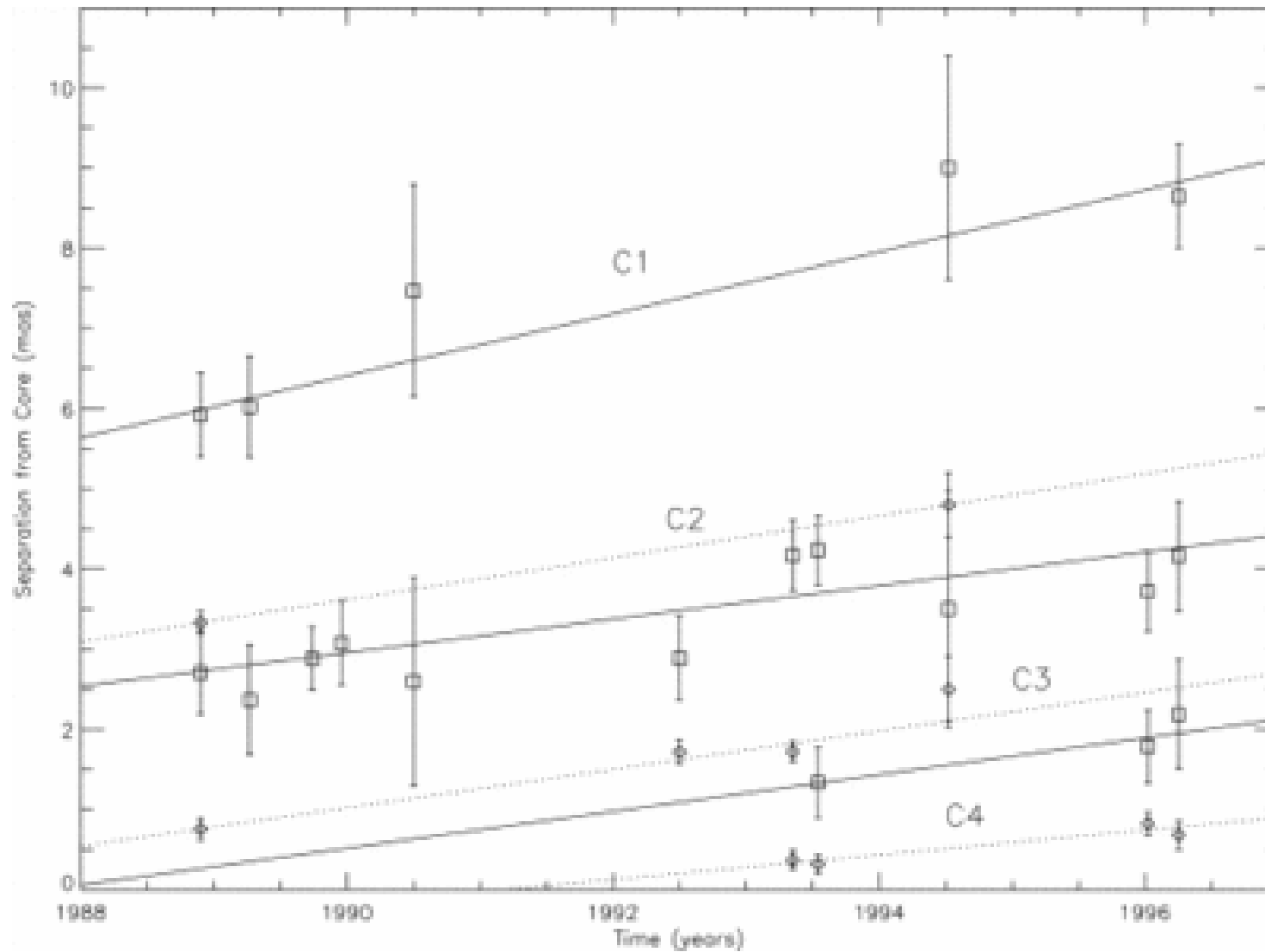
Fig. 2. from A Slower Superluminal Velocity for the Quasar 1156+295 Piner & Kingham 1997 ApJL 485 L61 doi:10.1086/310820 https://dx.doi.org/10.1086/310820 ©1997. The American Astronomical Society. All rights reserved. Printed in U.S.A.
