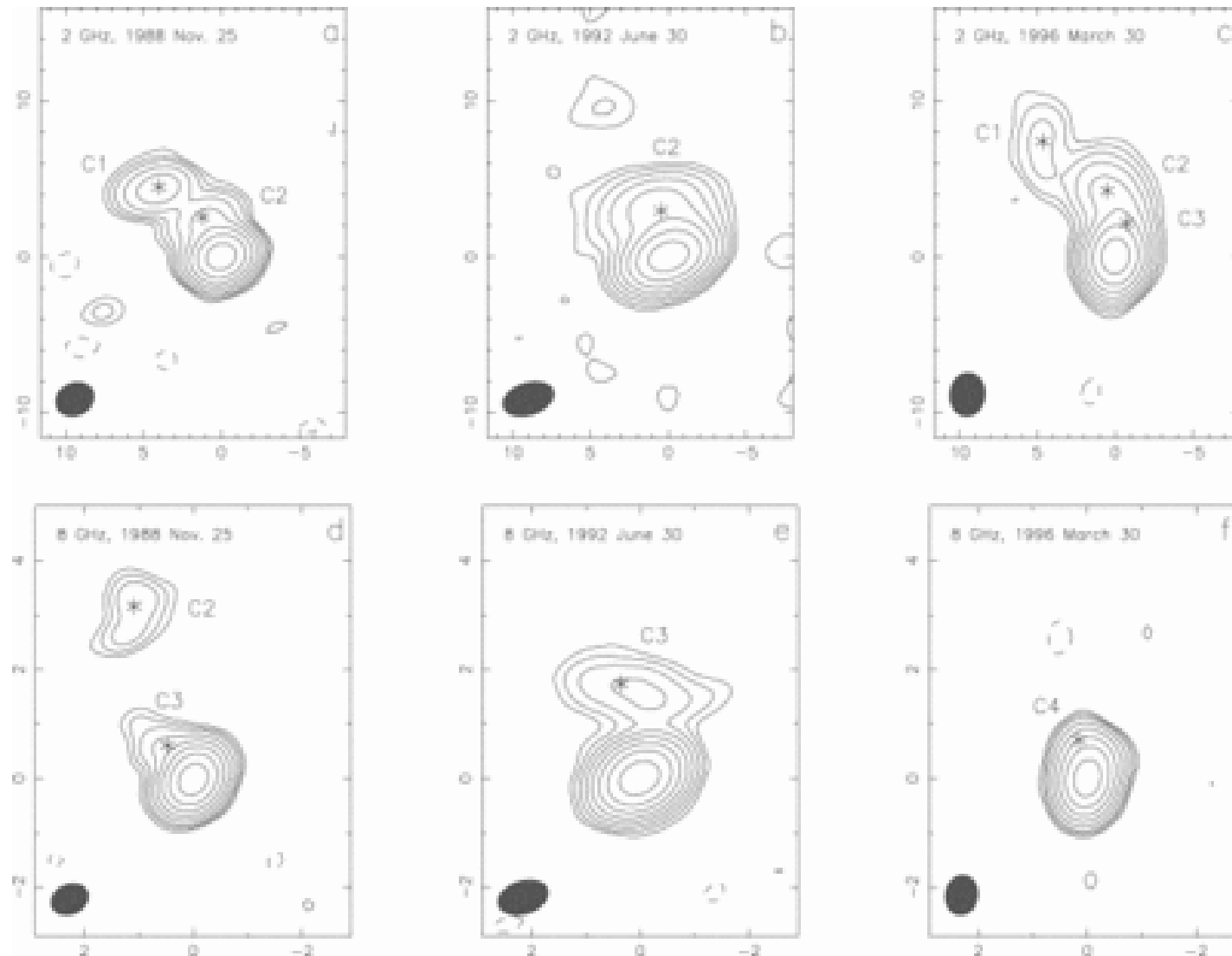
Fig. 1. from A Slower Superluminal Velocity for the Quasar 1156+295 Piner & Kingham 1997 ApJL 485 L61 doi:10.1086/310820 https://dx.doi.org/10.1086/310820 ©1997. The American Astronomical Society. All rights reserved. Printed in U.S.A.
