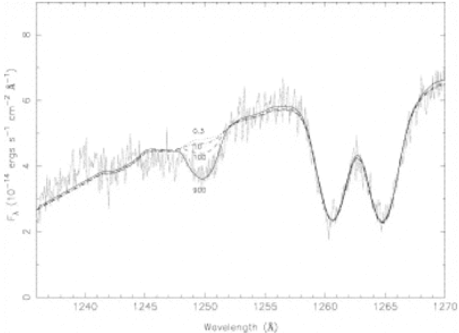
Fig. 2. from Evidence of a Thermonuclear Runaway and Proton Capture Material on a White Dwarf in a Dwarf Nova Sion et al. 1997 ApJL 480 L17 doi:10.1086/310623 https://dx.doi.org/10.1086/310623 ©1997. The American Astronomical Society. All rights reserved. Printed in U.S.A.
