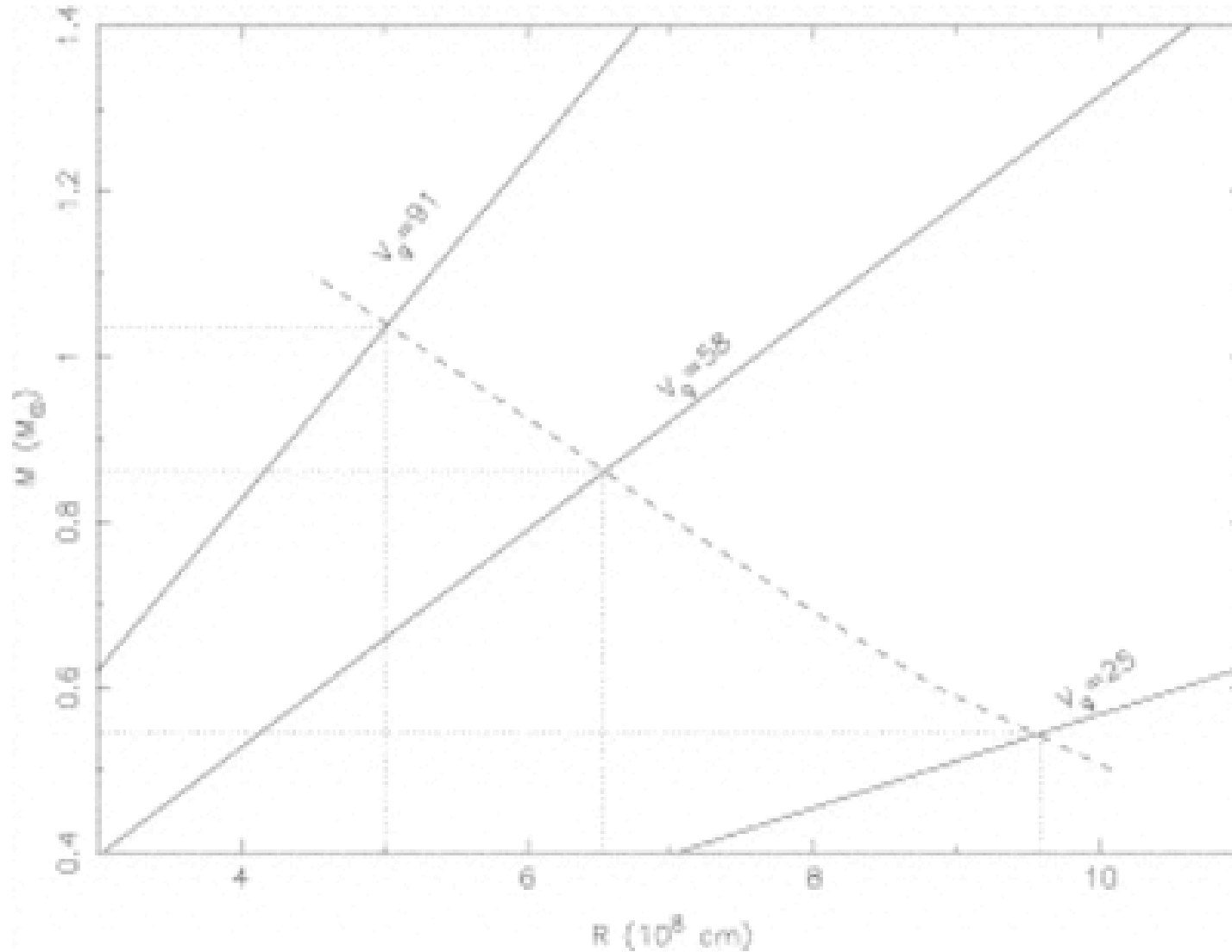
Fig. 1. from Evidence of a Thermonuclear Runaway and Proton Capture Material on a White Dwarf in a Dwarf Nova Sion et al. 1997 ApJL 480 L17 doi:10.1086/310623 https://dx.doi.org/10.1086/310623 ©1997. The American Astronomical Society. All rights reserved. Printed in U.S.A.
