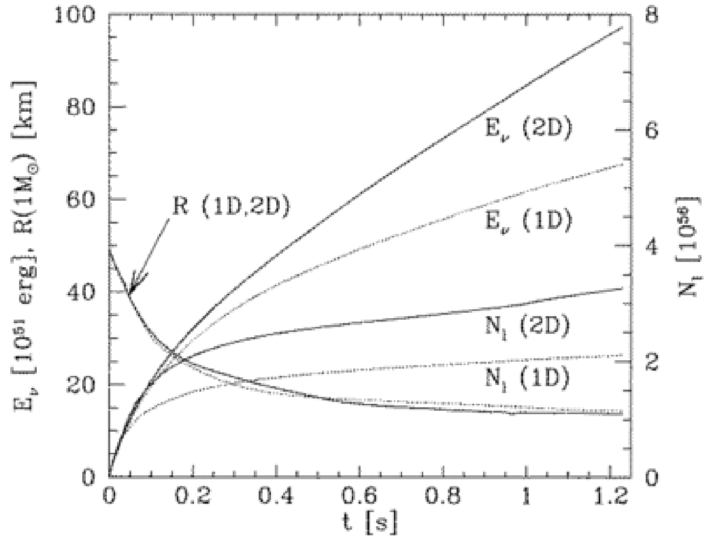
Fig. 4. from Ledoux Convection in Protoneutron Stars—A Clue to Supernova Nucleosynthesis? Keil, Janka, & Müller 1996 ApJL 473 L111 doi:10.1086/310404 https://dx.doi.org/10.1086/310404 ©1996. The American Astronomical Society. All rights reserved. Printed in U.S.A.
