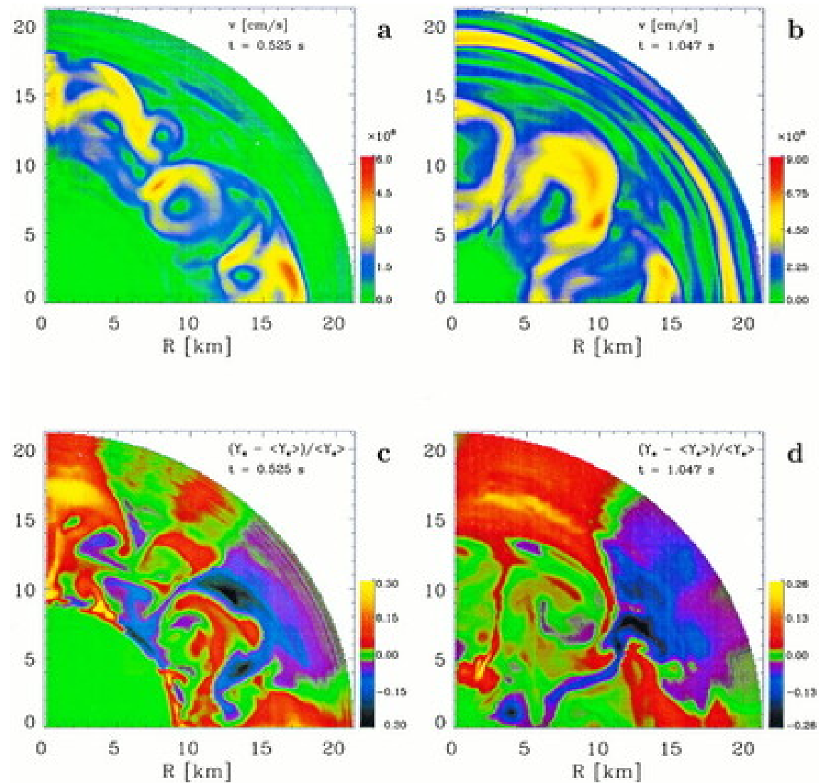
Fig. 3. from Ledoux Convection in Protoneutron Stars—A Clue to Supernova Nucleosynthesis? Keil, Janka, & Müller 1996 ApJL 473 L111 doi:10.1086/310404 https://dx.doi.org/10.1086/310404 ©1996. The American Astronomical Society. All rights reserved. Printed in U.S.A.
