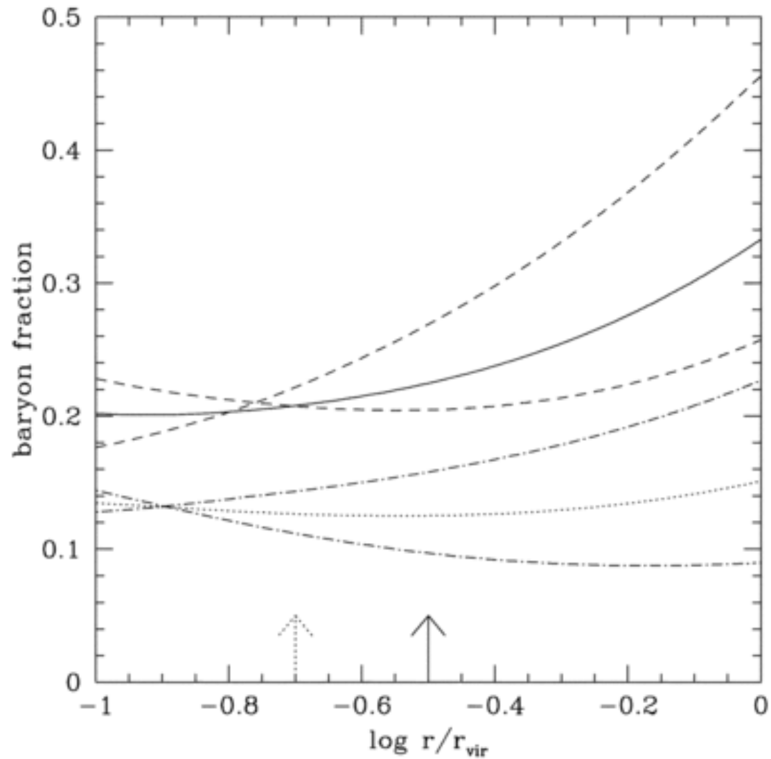
Fig. 2. from The Mass of Abell 1060 and AWM 7 from Spatially Resolved XRay Spectroscopy: Variations in Baryon Fraction Loewenstein & Mushotzky 1996 ApJL 471 L83 doi:10.1086/310342 https://dx.doi.org/10.1086/310342 ©1996. The American Astronomical Society. All rights reserved. Printed in U.S.A.
