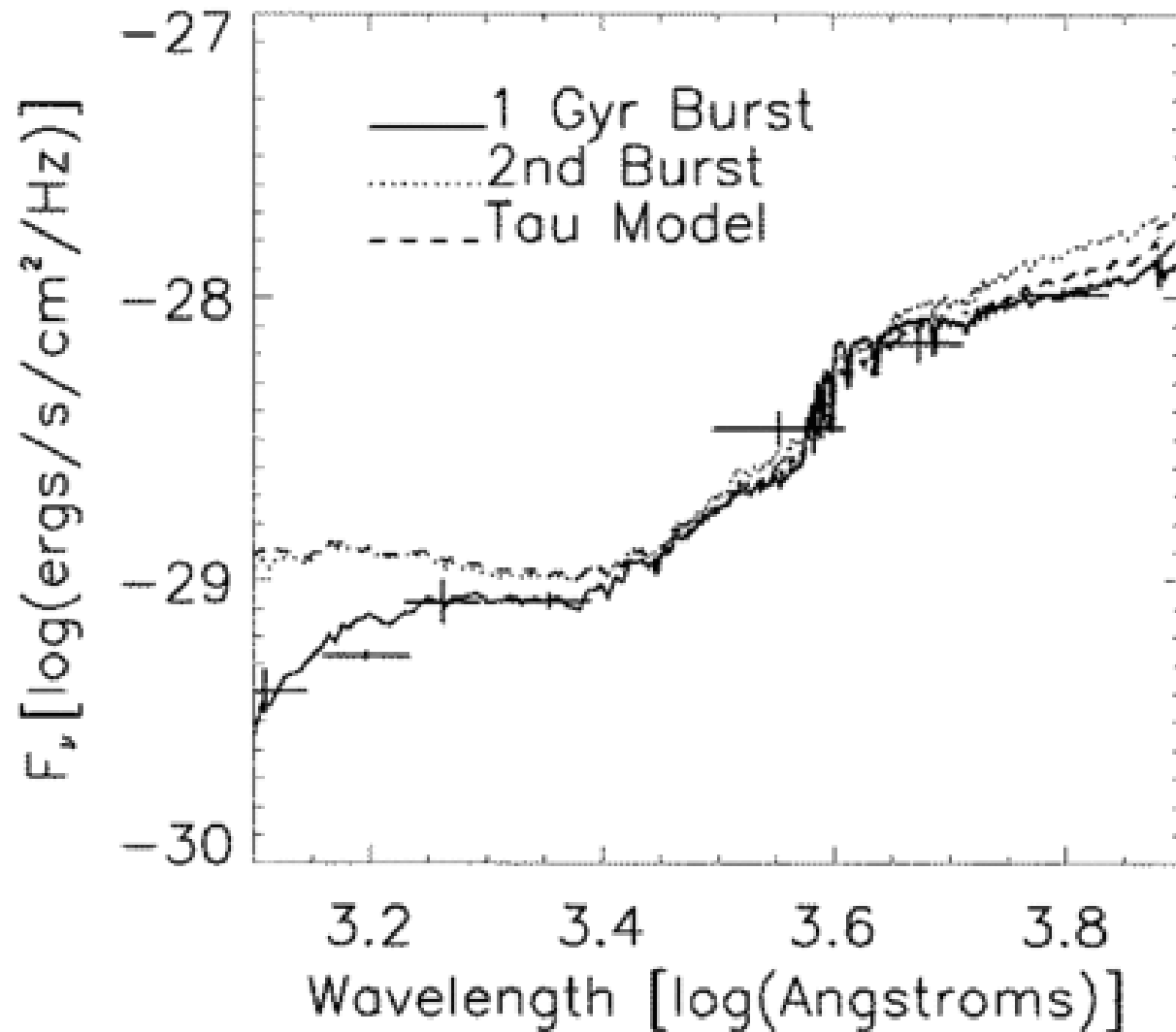
Fig. 2. from A Young Cluster of Galaxies at z = 2.5 Malkan, Teplitz, & McLean 1996 ApJL 468 L9 doi:10.1086/310228 https://dx.doi.org/10.1086/310228 ©1996. The American Astronomical Society. All rights reserved. Printed in U.S.A.
