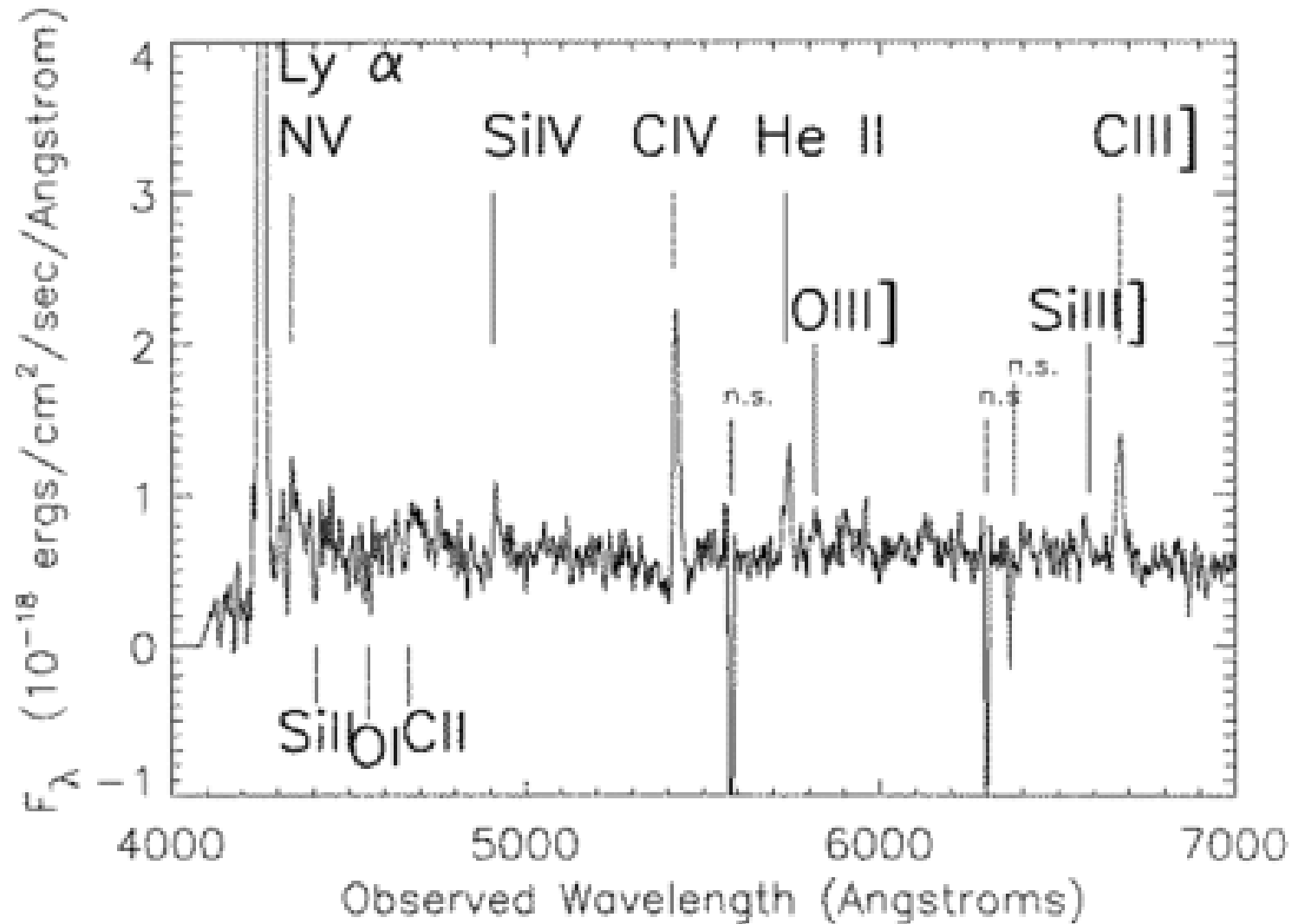
Fig. 1. from A Young Cluster of Galaxies at z = 2.5 Malkan, Teplitz, & McLean 1996 ApJL 468 L9 doi:10.1086/310228 https://dx.doi.org/10.1086/310228 ©1996. The American Astronomical Society. All rights reserved. Printed in U.S.A.
