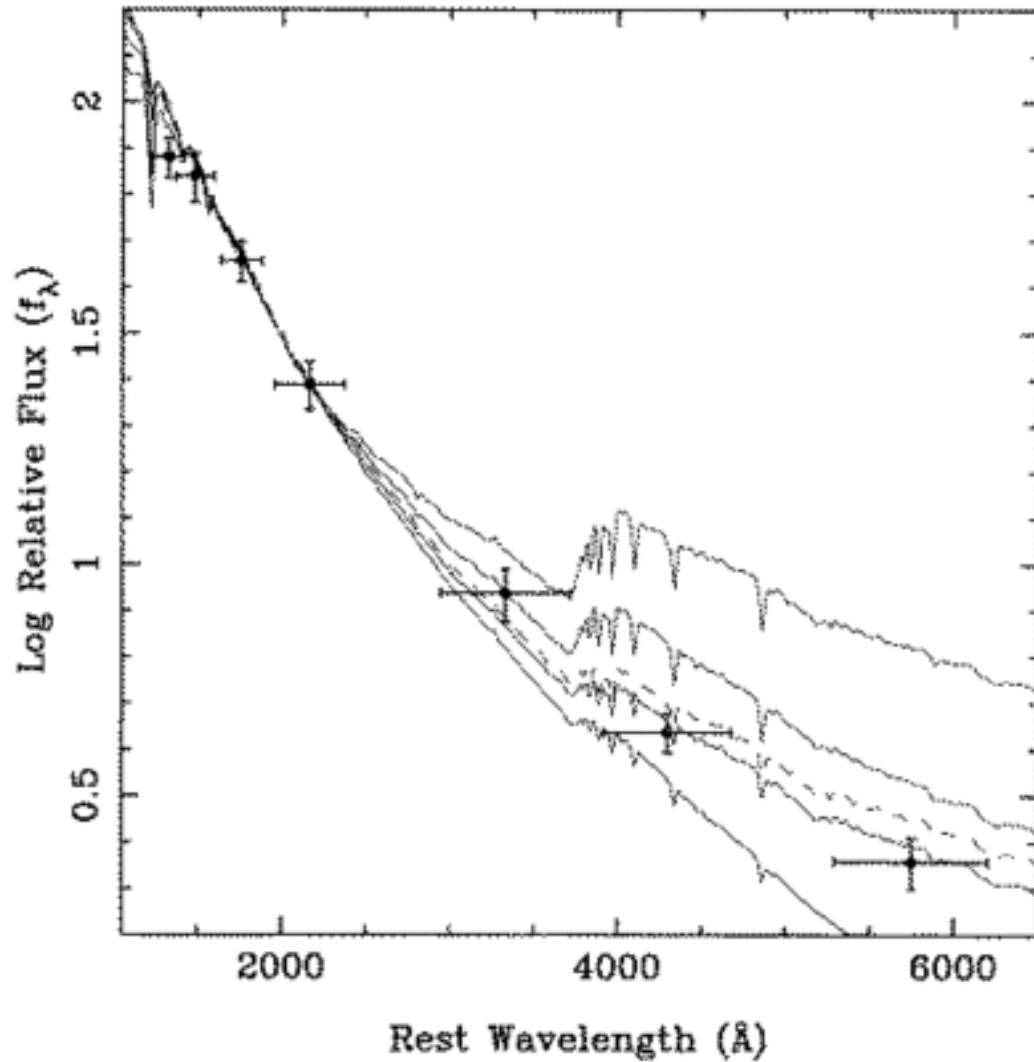
Fig. 3. from OpticalIR Spectral Energy Distribution of the Protogalaxy Candidate MS 1512cB58 Ellingson et al. 1996 ApJL 466 L71 doi:10.1086/310182 https://dx.doi.org/10.1086/310182 ©1996. The American Astronomical Society. All rights reserved. Printed in U.S.A.
