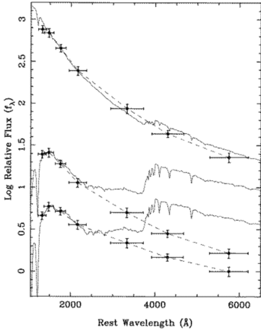
Fig. 2. from OpticalIR Spectral Energy Distribution of the Protogalaxy Candidate MS 1512cB58 Ellingson et al. 1996 ApJL 466 L71 doi:10.1086/310182 https://dx.doi.org/10.1086/310182 ©1996. The American Astronomical Society. All rights reserved. Printed in U.S.A.
