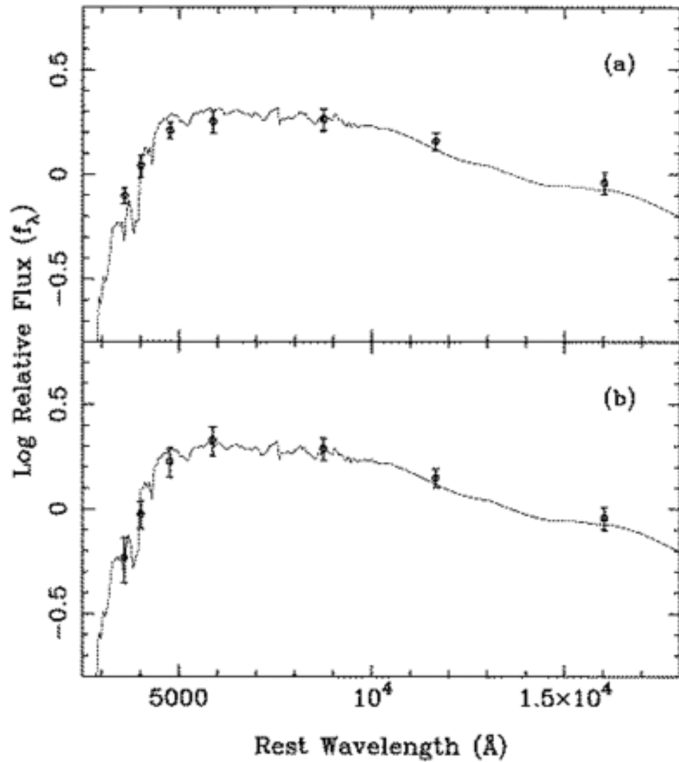
Fig. 1. from OpticalIR Spectral Energy Distribution of the Protogalaxy Candidate MS 1512cB58 Ellingson et al. 1996 ApJL 466 L71 doi:10.1086/310182 https://dx.doi.org/10.1086/310182 ©1996. The American Astronomical Society. All rights reserved. Printed in U.S.A.
