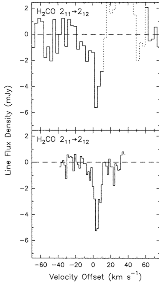
Fig. 2. from Formaldehyde Absorption at z = 0.685 toward the “Einstein Ring” B0218+357 Menten & Reid 1996 ApJL 465 L99 doi:10.1086/310147 https://dx.doi.org/10.1086/310147 ©1996. The American Astronomical Society. All rights reserved. Printed in U.S.A.
