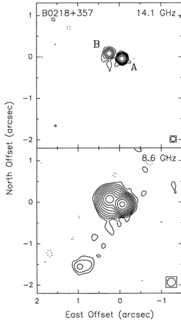
Fig. 1. from Formaldehyde Absorption at z = 0.685 toward the “Einstein Ring” B0218+357 Menten & Reid 1996 ApJL 465 L99 doi:10.1086/310147 https://dx.doi.org/10.1086/310147 ©1996. The American Astronomical Society. All rights reserved. Printed in U.S.A.
