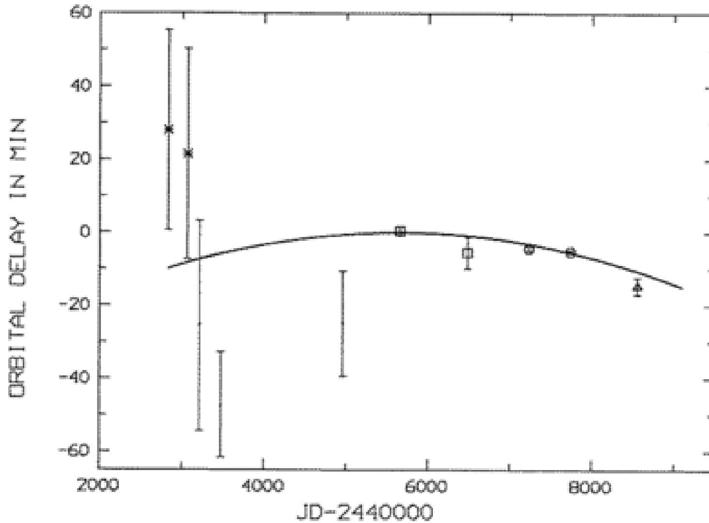
Fig. 4. from Orbital Decay in the XRay Binary LMC X4 SafiHarb, Ögelman, & Dennerl 1996 ApJL 456 L37 doi:10.1086/309859 https://dx.doi.org/10.1086/309859 © 1996. The American Astronomical Society. All rights reserved. Printed in U.S.A.
