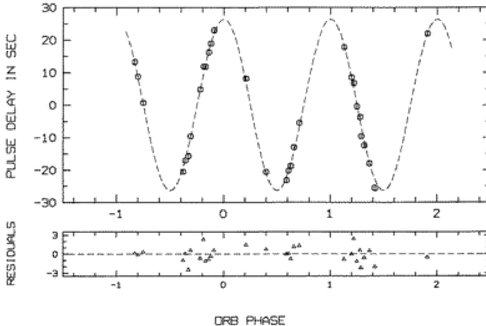
Fig. 3. from Orbital Decay in the XRay Binary LMC X4 SafiHarb, Ögelman, & Dennerl 1996 ApJL 456 L37 doi:10.1086/309859 https://dx.doi.org/10.1086/309859 © 1996. The American Astronomical Society. All rights reserved. Printed in U.S.A.
