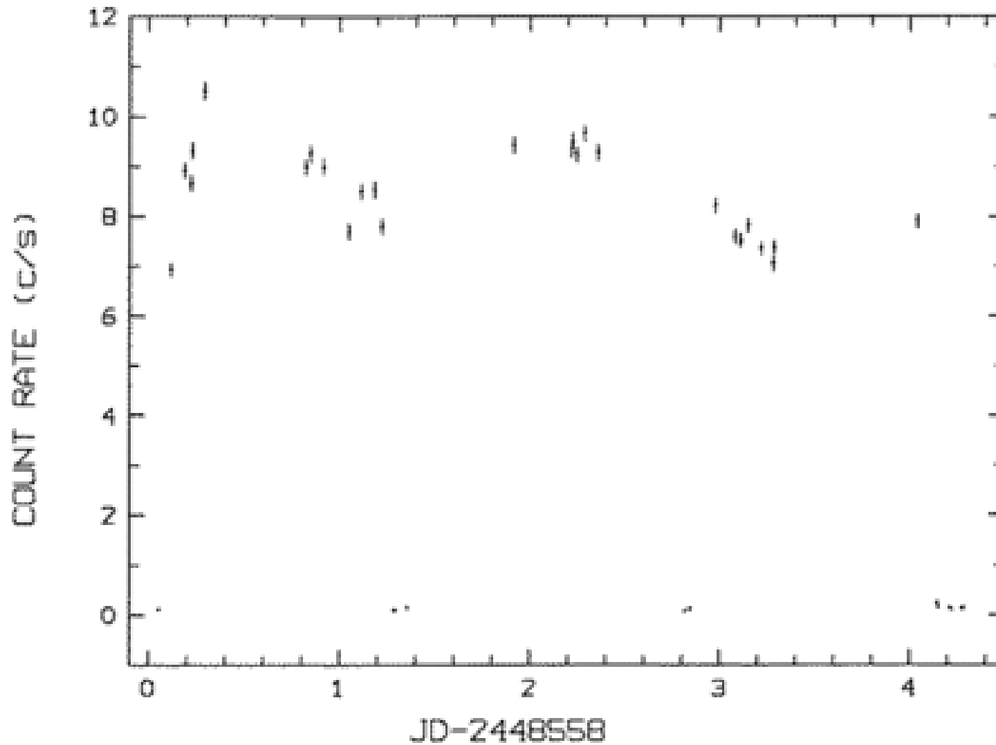
Fig. 1. from Orbital Decay in the XRay Binary LMC X4 SafiHarb, Ögelman, & Dennerl 1996 ApJL 456 L37 doi:10.1086/309859 https://dx.doi.org/10.1086/309859 © 1996. The American Astronomical Society. All rights reserved. Printed in U.S.A.
