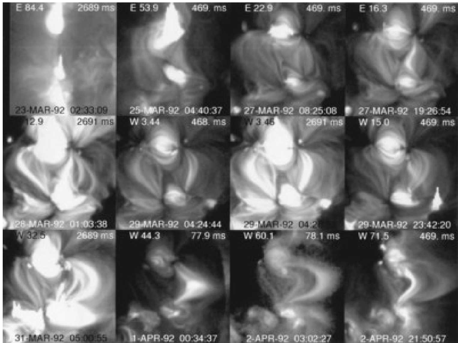
Fig. 2. from Interacting Active Regions in the Solar Corona Tsuneta 1996 ApJL 456 L63 doi:10.1086/309857 https://dx.doi.org/10.1086/309857 © 1996. The American Astronomical Society. All rights reserved. Printed in U.S.A.
