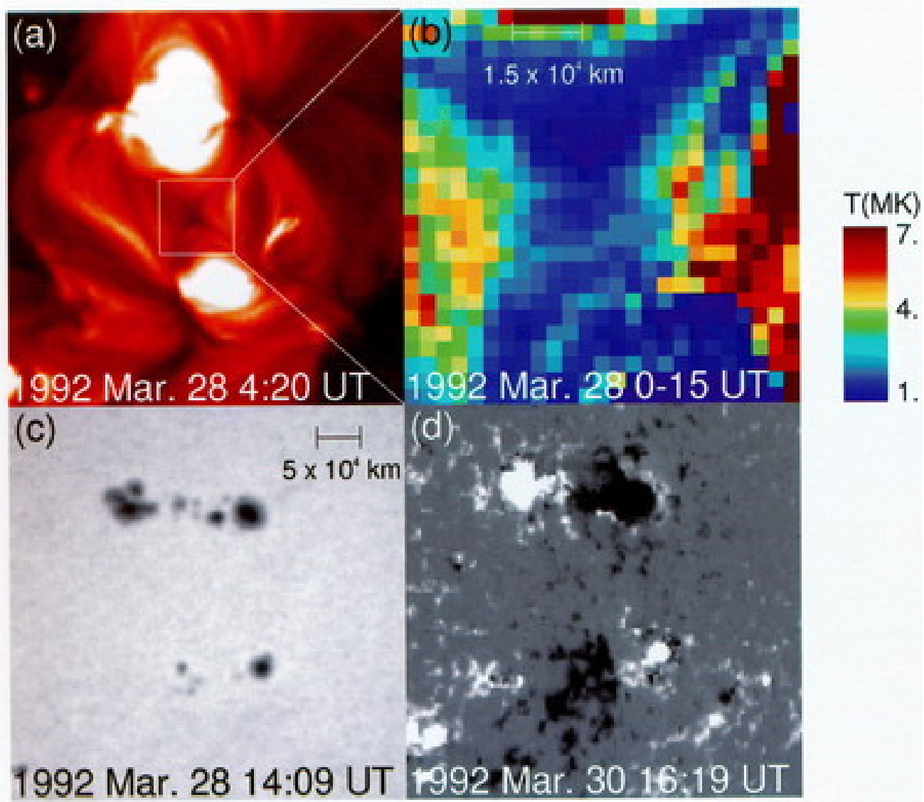
Fig. 1. from Interacting Active Regions in the Solar Corona Tsuneta 1996 ApJL 456 L63 doi:10.1086/309857 https://dx.doi.org/10.1086/309857 © 1996. The American Astronomical Society. All rights reserved. Printed in U.S.A.
