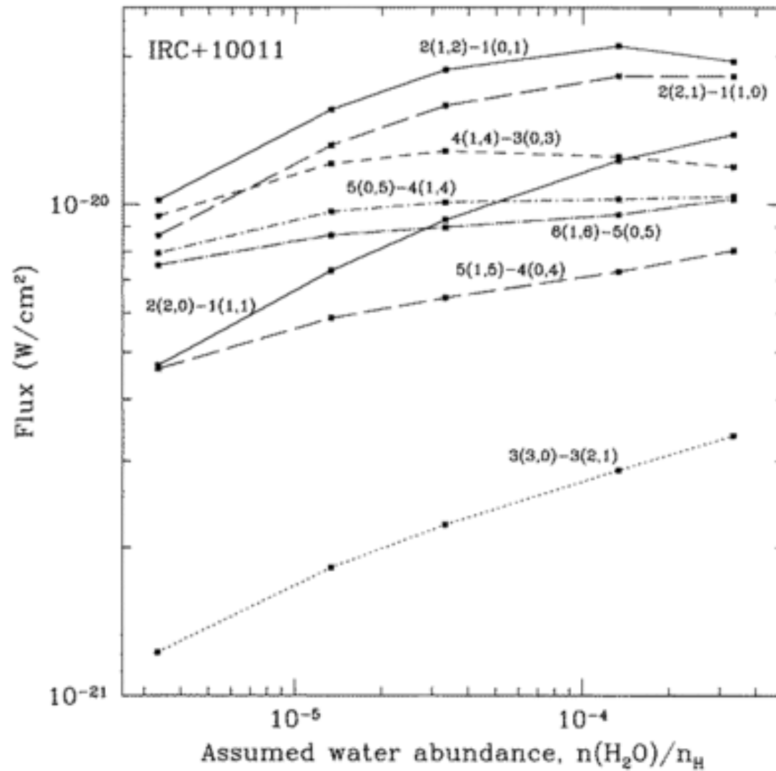
Fig. 4. from FarInfrared Water Line Emissions from Circumstellar Outflows Chen & Neufeld 1995 ApJL 453 L99 doi:10.1086/309745 https://dx.doi.org/10.1086/309745 © 1995. The American Astronomical Society. All rights reserved. Printed in U.S.A.
