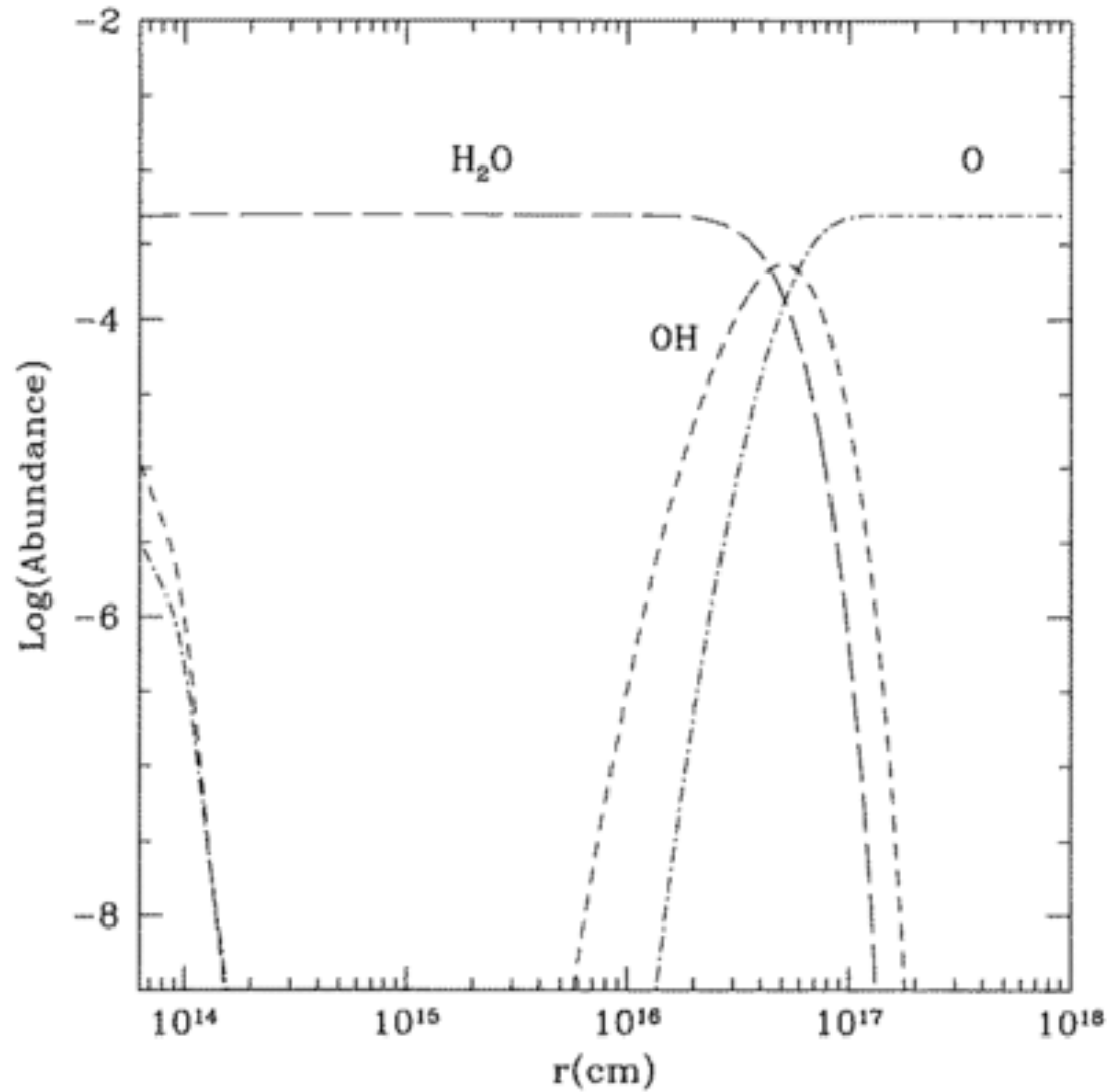
Fig. 2. from FarInfrared Water Line Emissions from Circumstellar Outflows Chen & Neufeld 1995 ApJL 453 L99 doi:10.1086/309745 https://dx.doi.org/10.1086/309745 © 1995. The American Astronomical Society. All rights reserved. Printed in U.S.A.
