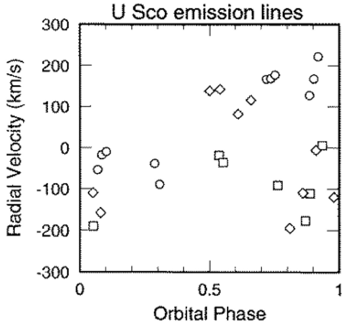
Fig. 2. from An Improved Orbital Period for the Recurrent Nova U Scorpii Schaefer & Ringwald 1995 ApJL 447 L45 doi:10.1086/309550 https://dx.doi.org/10.1086/309550 © 1995. The American Astronomical Society. All rights reserved. Printed in U.S.A.
