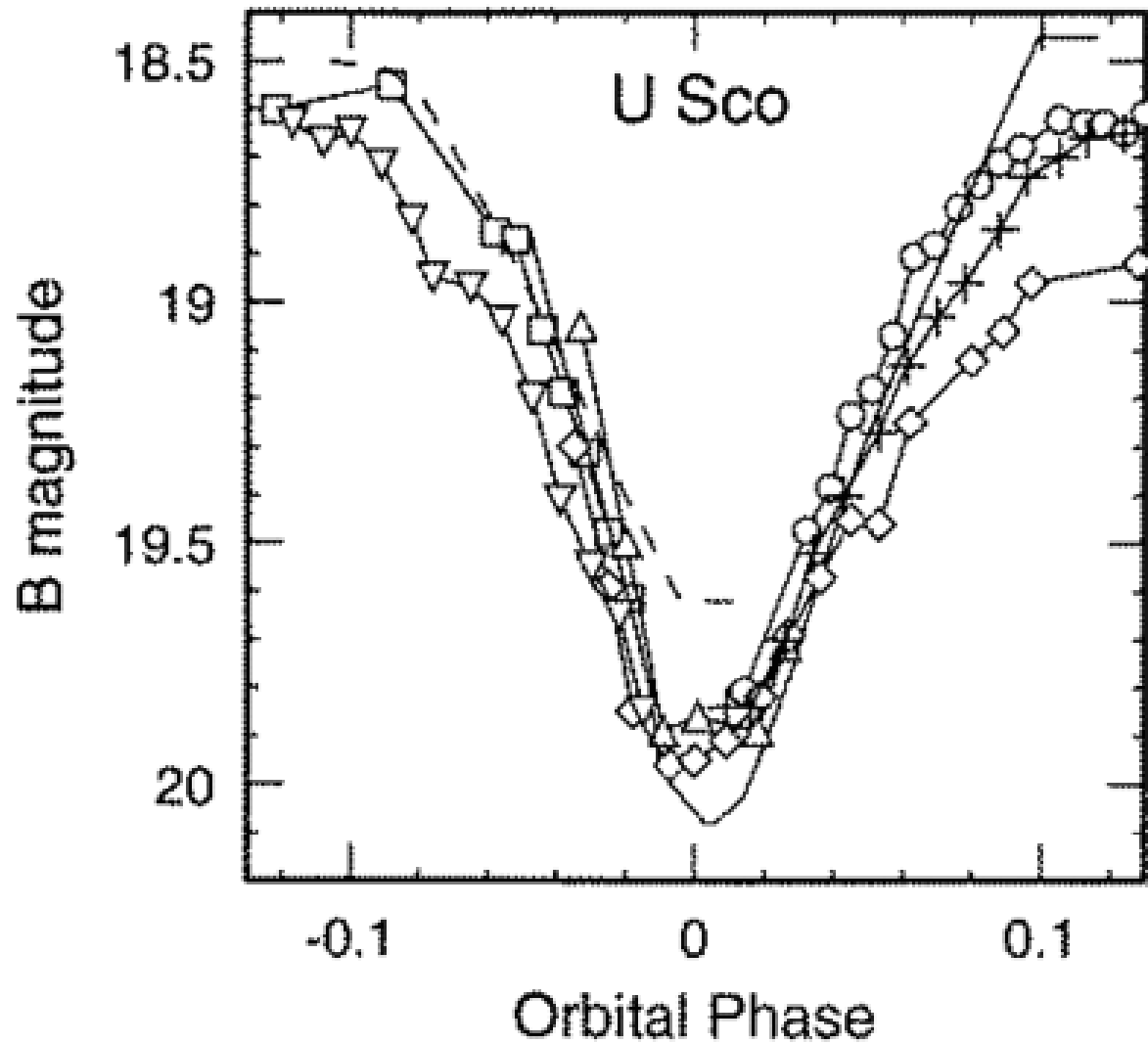
Fig. 1. from An Improved Orbital Period for the Recurrent Nova U Scorpii Schaefer & Ringwald 1995 ApJL 447 L45 doi:10.1086/309550 https://dx.doi.org/10.1086/309550 © 1995. The American Astronomical Society. All rights reserved. Printed in U.S.A.
