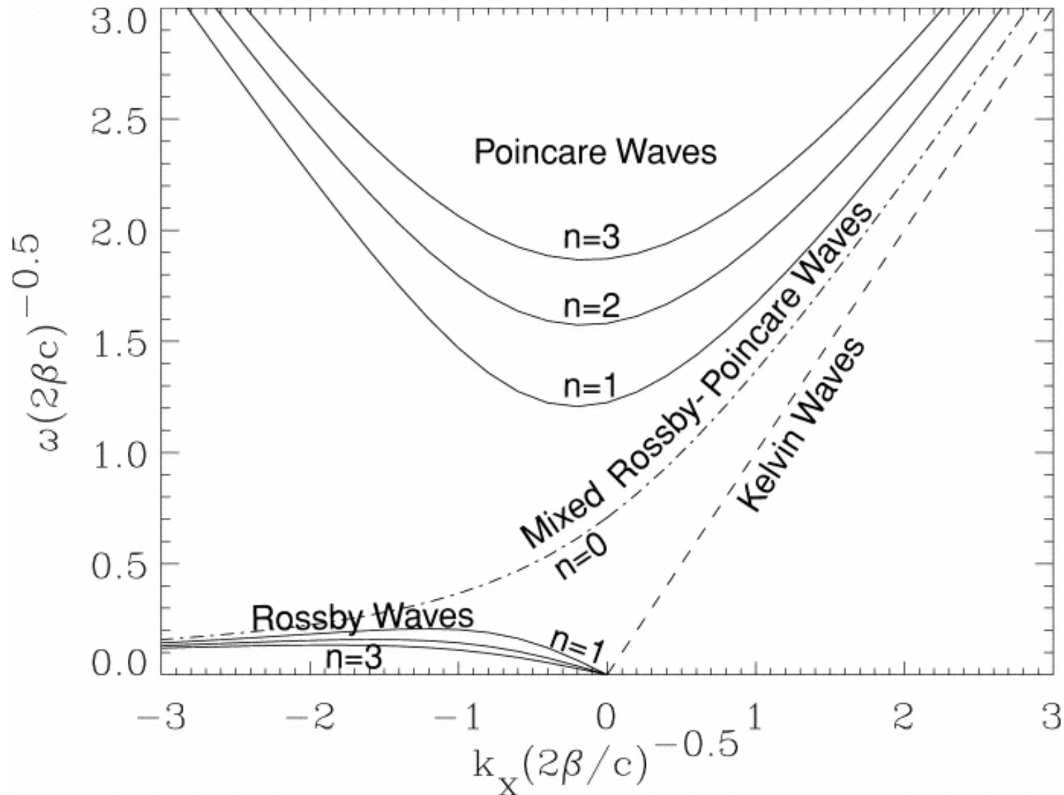
Fig. 1. from RossbyType Wave–Induced Periodicities in Flare Activities and Sunspot Areas or Groups during Solar Maxima Lou 2000 ApJ 540 1102 doi:10.1086/309387 https://dx.doi.org/10.1086/309387 © 2000. The American Astronomical Society. All rights reserved. Printed in U.S.A.
