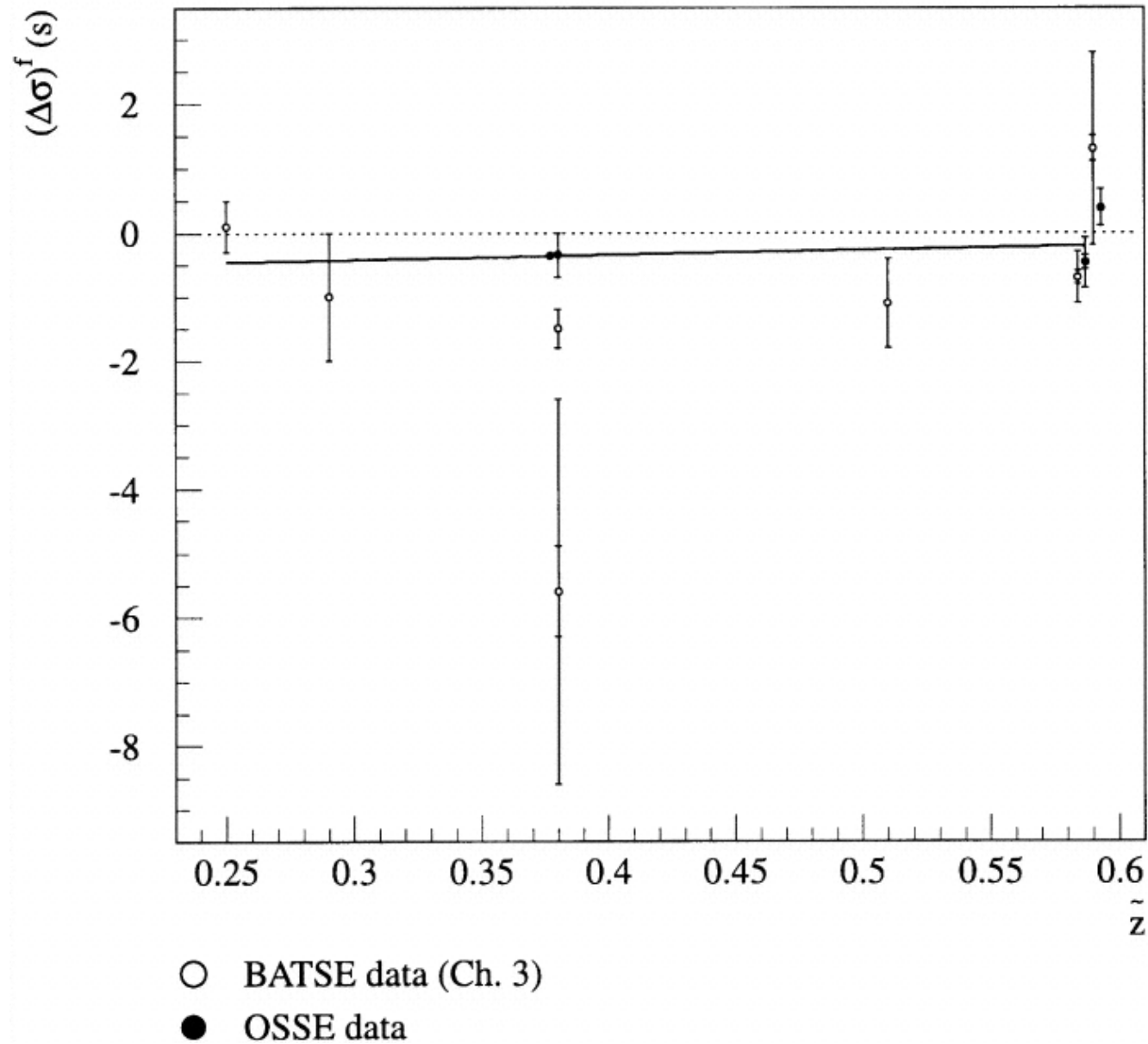
Fig. 9. from A Search in GammaRay Burst Data for Nonconstancy of the Velocity of Light Ellis et al. 2000 ApJ 535 139 doi:10.1086/308825 https://dx.doi.org/10.1086/308825 © 2000. The American Astronomical Society. All rights reserved. Printed in U.S.A.
