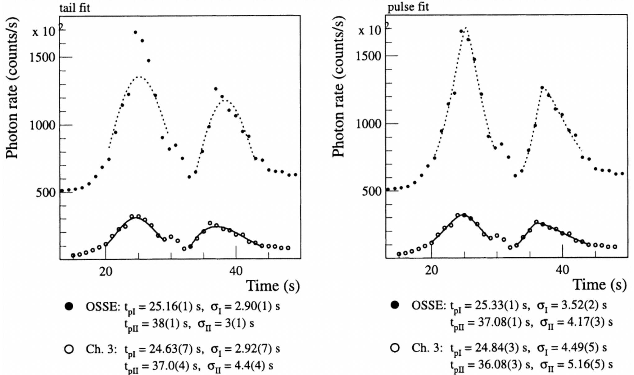
Fig. 7. from A Search in GammaRay Burst Data for Nonconstancy of the Velocity of Light Ellis et al. 2000 ApJ 535 139 doi:10.1086/308825 https://dx.doi.org/10.1086/308825 © 2000. The American Astronomical Society. All rights reserved. Printed in U.S.A.
