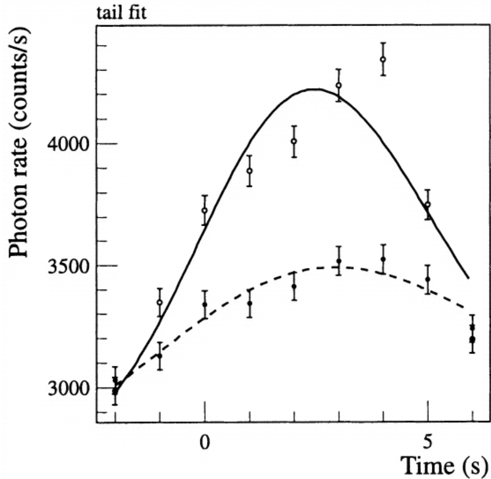
Fig. 2. from A Search in GammaRay Burst Data for Nonconstancy of the Velocity of Light Ellis et al. 2000 ApJ 535 139 doi:10.1086/308825 https://dx.doi.org/10.1086/308825 © 2000. The American Astronomical Society. All rights reserved. Printed in U.S.A.
