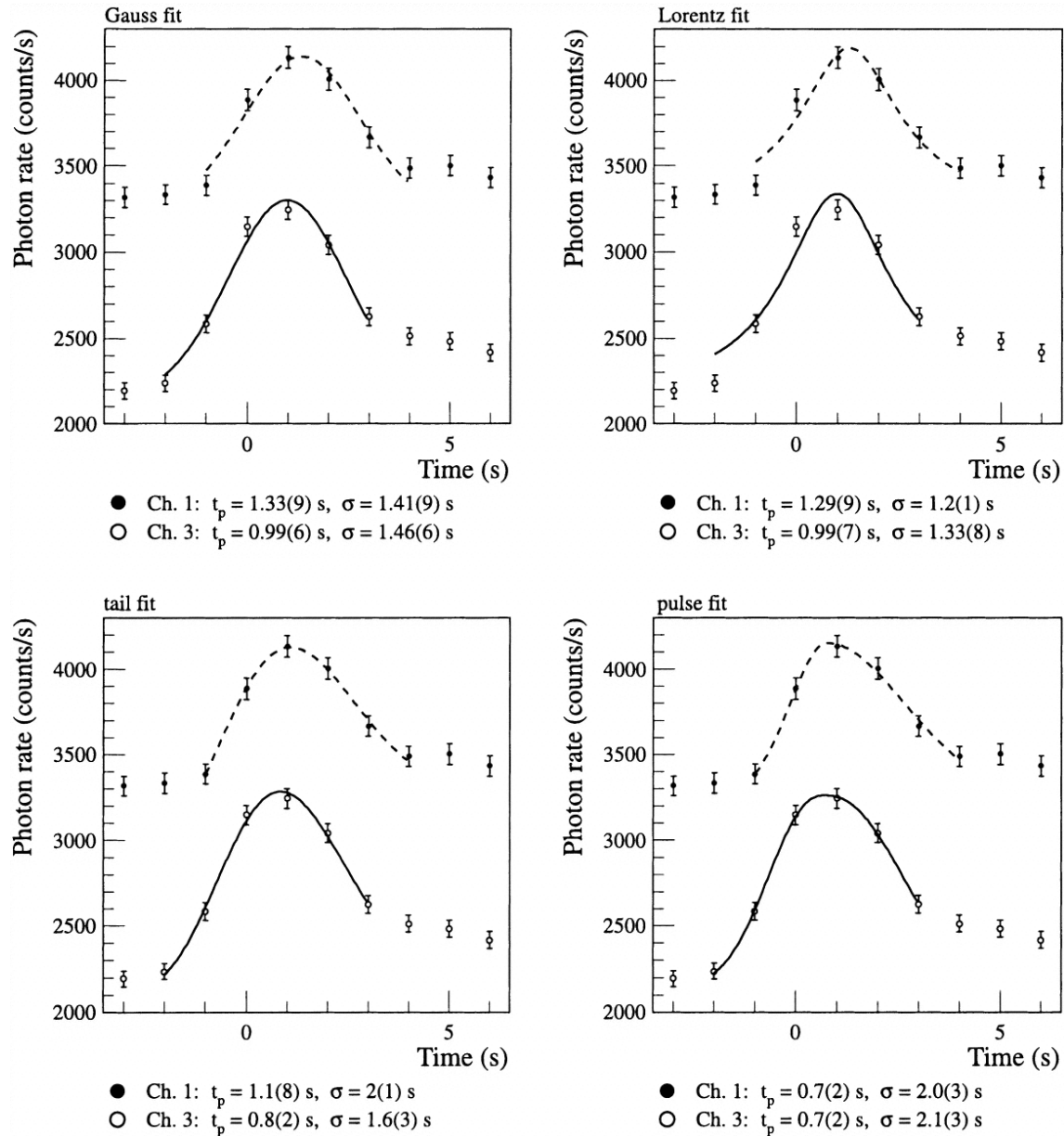
Fig. 1. from A Search in GammaRay Burst Data for Nonconstancy of the Velocity of Light Ellis et al. 2000 ApJ 535 139 doi:10.1086/308825 https://dx.doi.org/10.1086/308825
