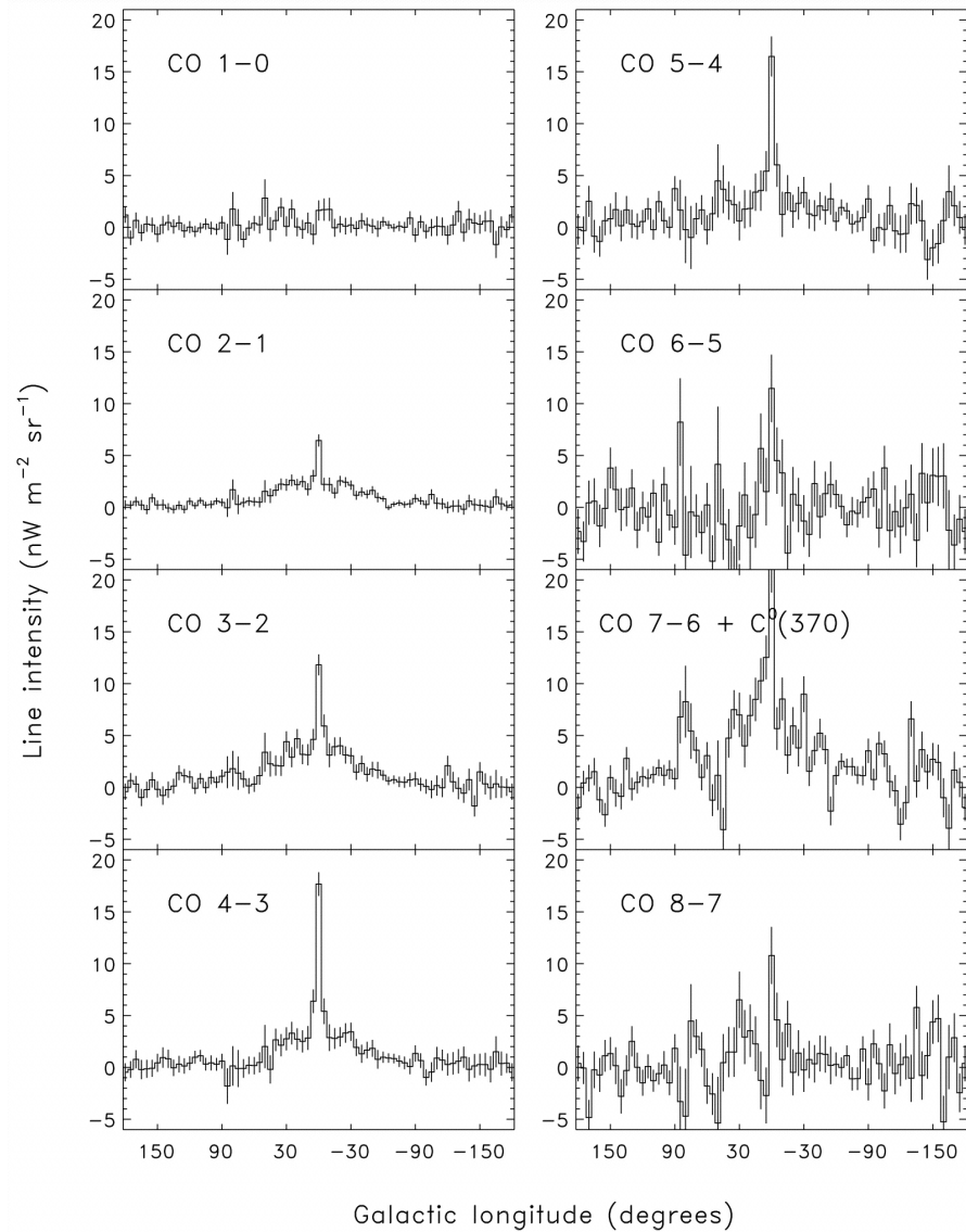
Fig. 3. from COBE Far Infrared Absolute Spectrophotometer Observations of Galactic Lines Fixsen, Bennett, & Mather 1999 ApJ 526 207 doi:10.1086/307962 https://dx.doi.org/10.1086/307962 © 1999. The American Astronomical Society. All rights reserved. Printed in U.S.A.
