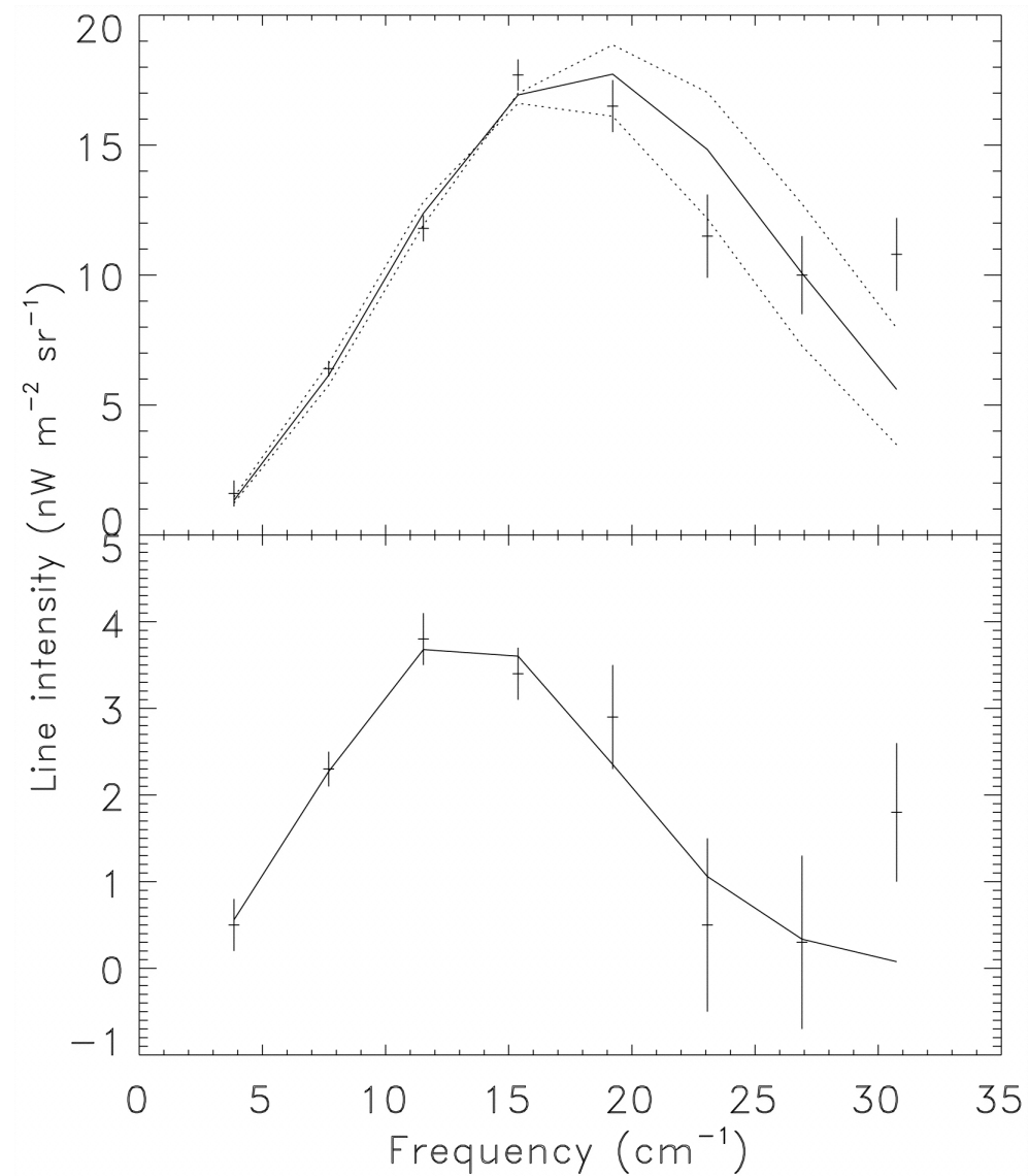
Fig. 2. from COBE Far Infrared Absolute Spectrophotometer Observations of Galactic Lines Fixsen, Bennett, & Mather 1999 ApJ 526 207 doi:10.1086/307962 https://dx.doi.org/10.1086/307962 © 1999. The American Astronomical Society. All rights reserved. Printed in U.S.A.
