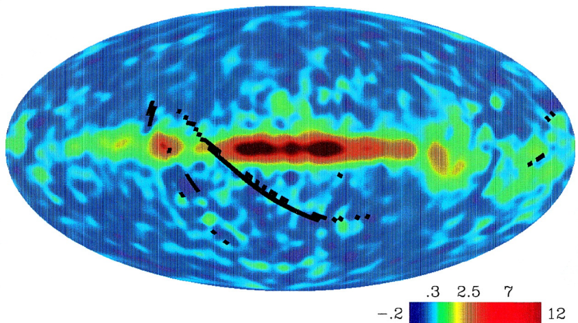
COBE FIRAS 205 \mu\text{m} N + Line Intensity
