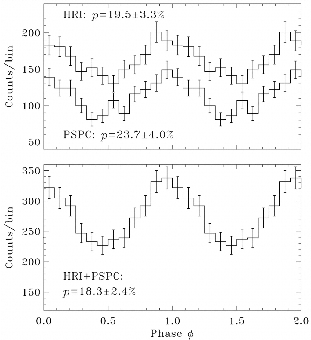
Fig. 8. from XRay Emission from the Radioquiet Neutron Star in Puppis A Zavlin, Trümper, & Pavlov 1999 ApJ 525 959 doi:10.1086/307919 https://dx.doi.org/10.1086/307919 © 1999. The American Astronomical Society. All rights reserved. Printed in U.S.A.
