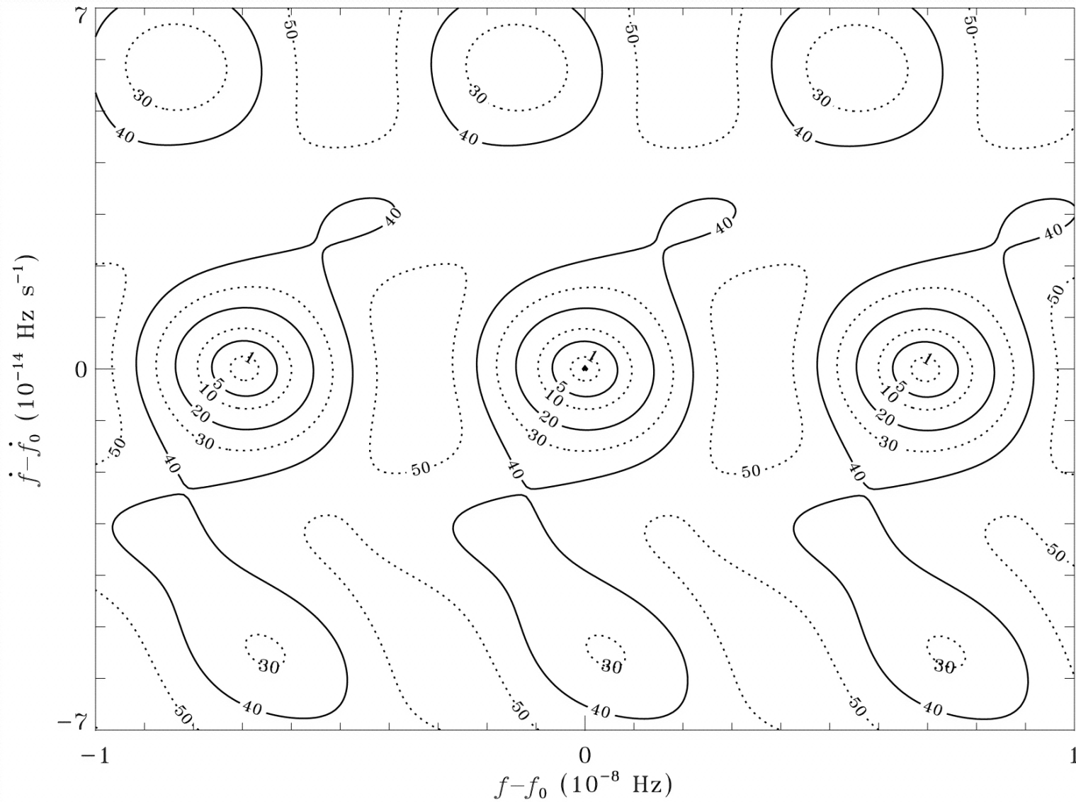
Fig. 7. from XRay Emission from the Radioquiet Neutron Star in Puppis A Zavlin, Trümper, & Pavlov 1999 ApJ 525 959 doi:10.1086/307919 https://dx.doi.org/10.1086/307919 © 1999. The American Astronomical Society. All rights reserved. Printed in U.S.A.
