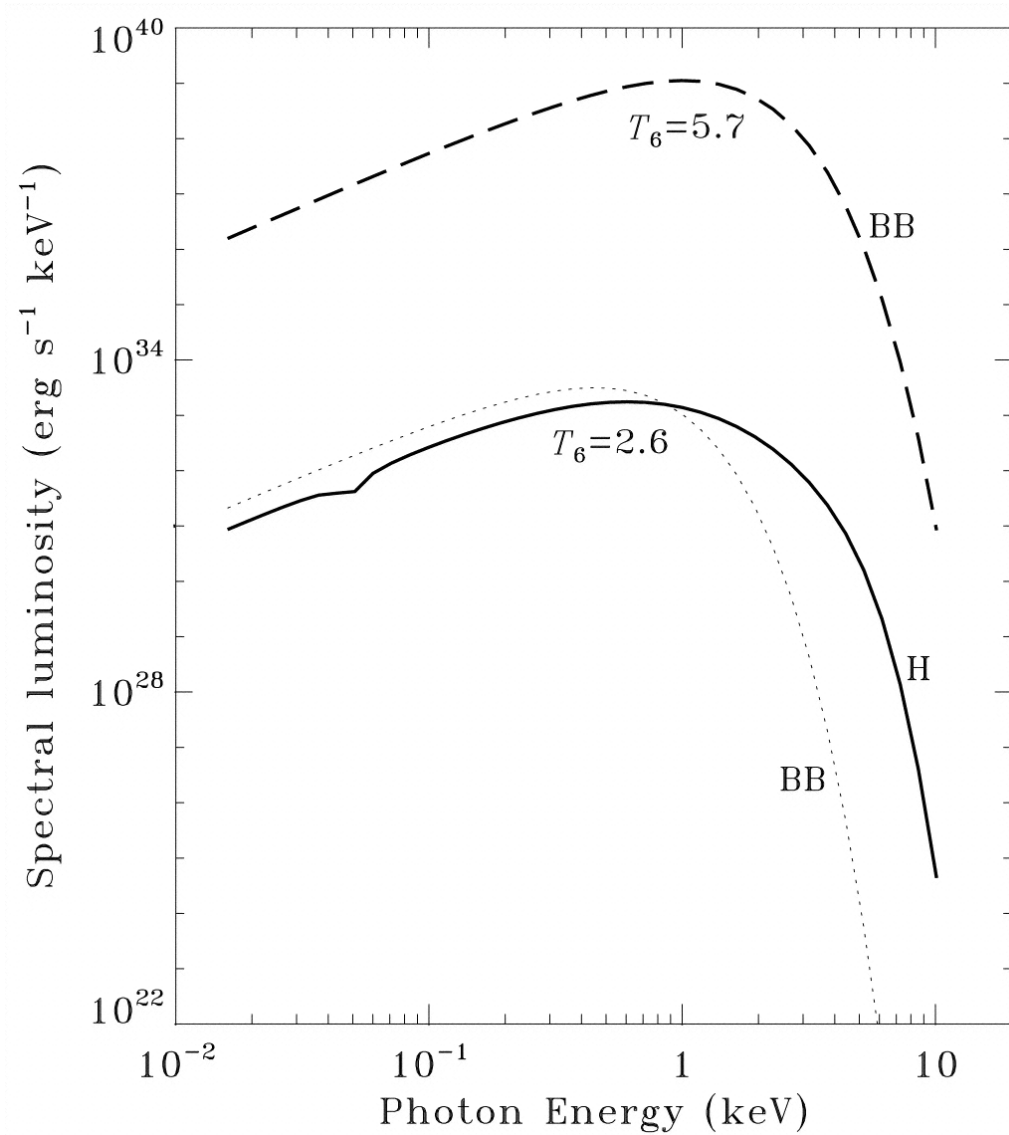
Fig. 5. from XRay Emission from the Radioquiet Neutron Star in Puppis A Zavlin, Trümper, & Pavlov 1999 ApJ 525 959 doi:10.1086/307919 https://dx.doi.org/10.1086/307919 © 1999. The American Astronomical Society. All rights reserved. Printed in U.S.A.
