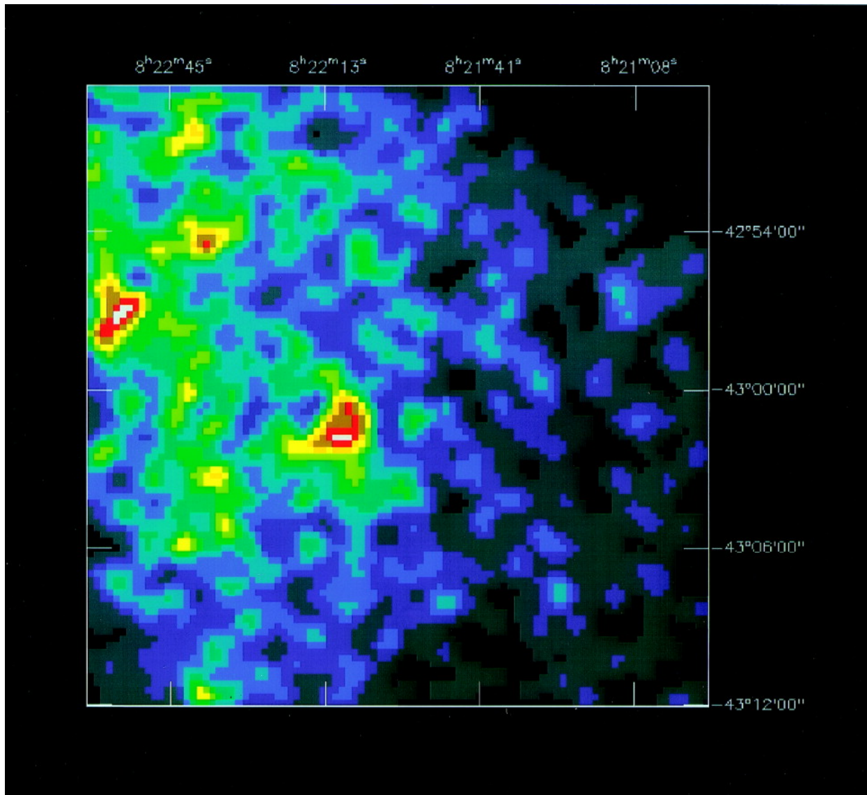
Fig. 1. from XRay Emission from the Radioquiet Neutron Star in Puppis A Zavlin, Trümper, & Pavlov 1999 ApJ 525 959 doi:10.1086/307919 https://dx.doi.org/10.1086/307919 © 1999. The American Astronomical Society. All rights reserved. Printed in U.S.A.
