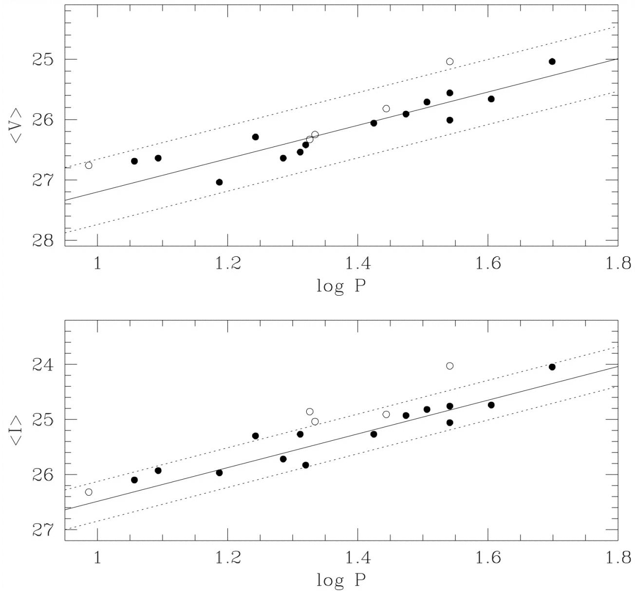
Fig. 7. from The Hubble Space Telescope Key Project on the Extragalactic Distance Scale. XXII. The Discovery of Cepheids in NGC 1326A Prosser et al. 1999 ApJ 525 80 doi:10.1086/307899 https://dx.doi.org/10.1086/307899 © 1999. The American Astronomical Society. All rights reserved. Printed in U.S.A.
