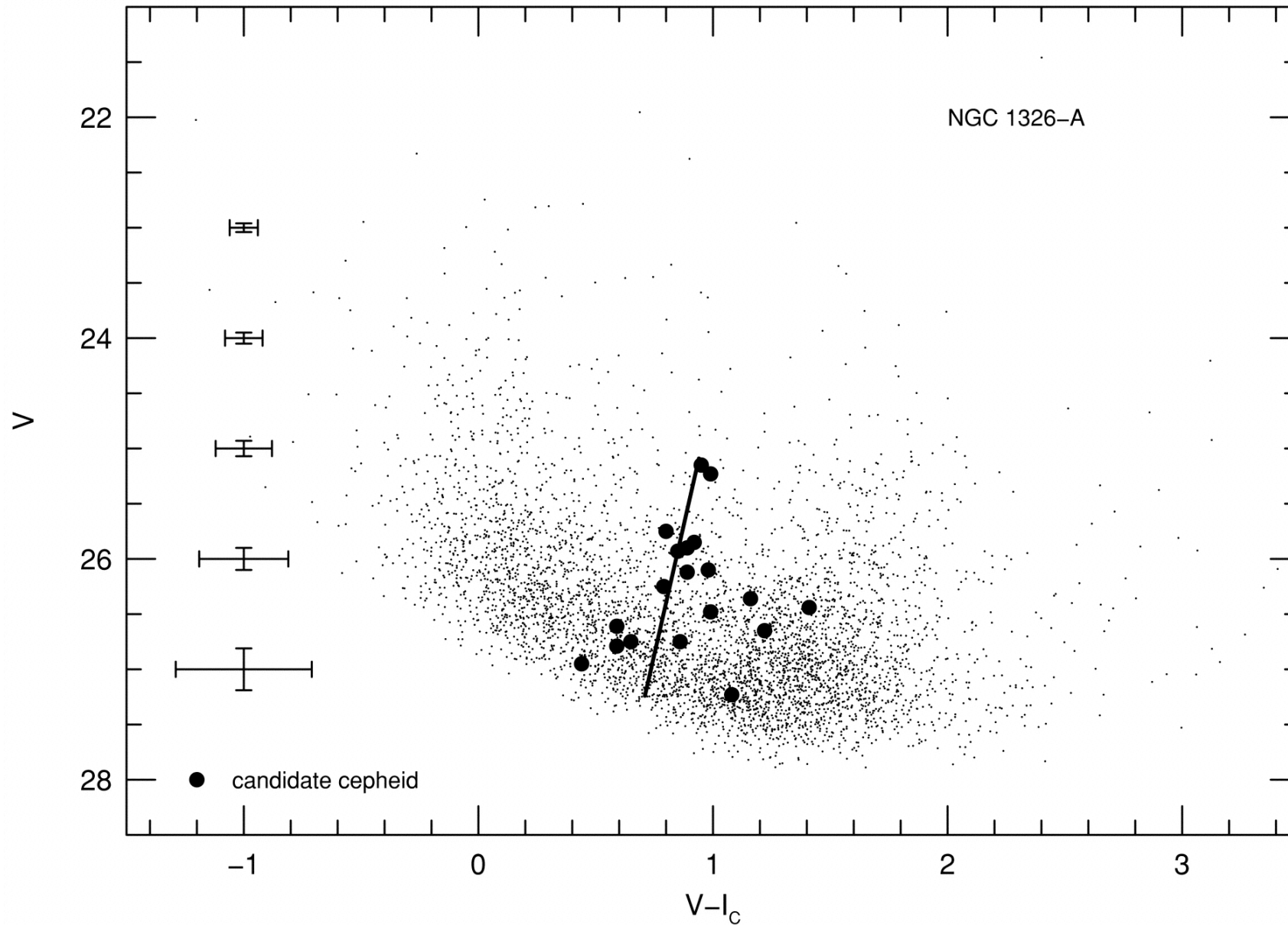
Fig. 6. from The Hubble Space Telescope Key Project on the Extragalactic Distance Scale. XXII. The Discovery of Cepheids in NGC 1326A Prosser et al. 1999 ApJ 525 80 doi:10.1086/307899 https://dx.doi.org/10.1086/307899 © 1999. The American Astronomical Society. All rights reserved. Printed in U.S.A.
