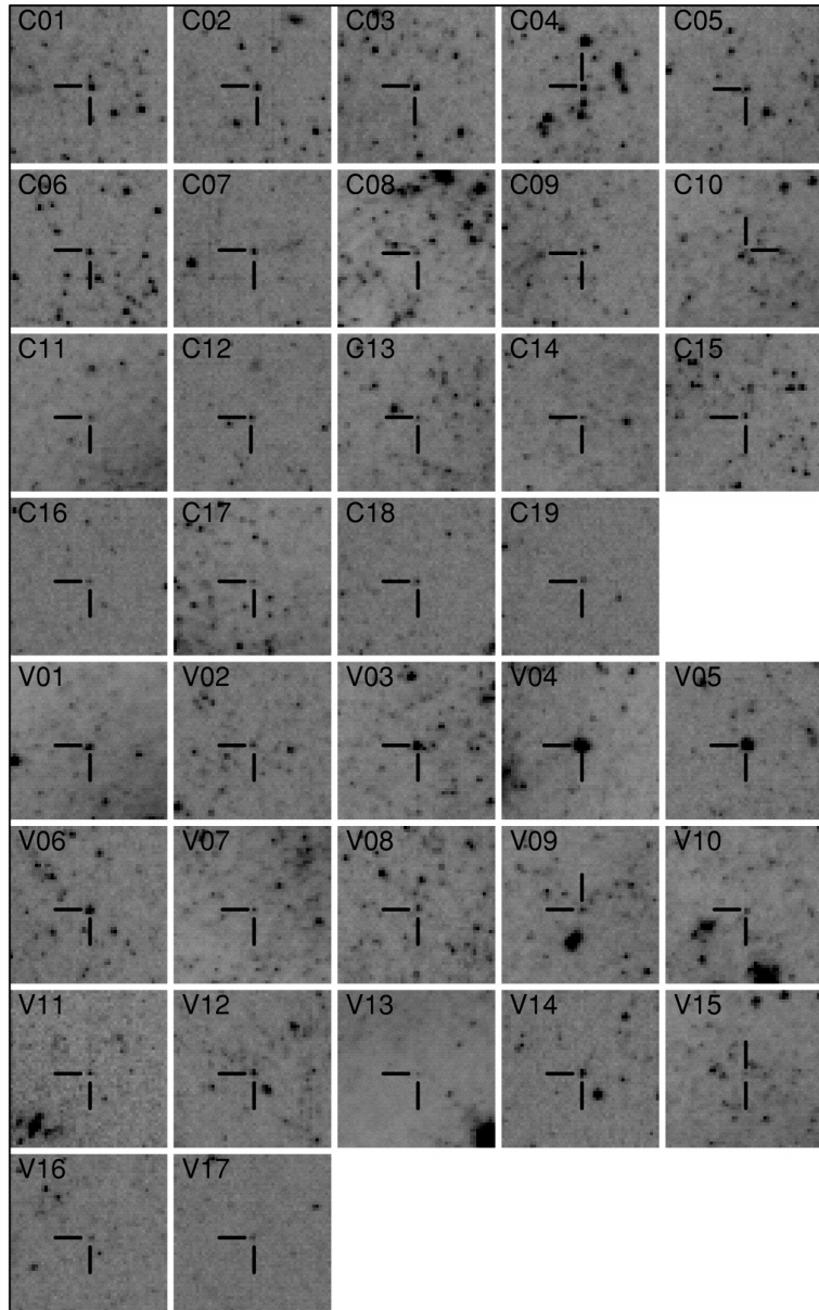
Fig. 4. from The Hubble Space Telescope Key Project on the Extragalactic Distance Scale. XXII. The Discovery of Cepheids in NGC 1326A Prosser et al. 1999 ApJ 525 80 doi:10.1086/307899 https://dx.doi.org/10.1086/307899
