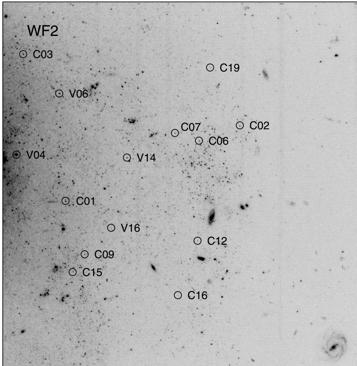
Fig. 3. from The Hubble Space Telescope Key Project on the Extragalactic Distance Scale. XXII. The Discovery of Cepheids in NGC 1326A Prosser et al. 1999 ApJ 525 80 doi:10.1086/307899 https://dx.doi.org/10.1086/307899 © 1999. The American Astronomical Society. All rights reserved. Printed in U.S.A.
