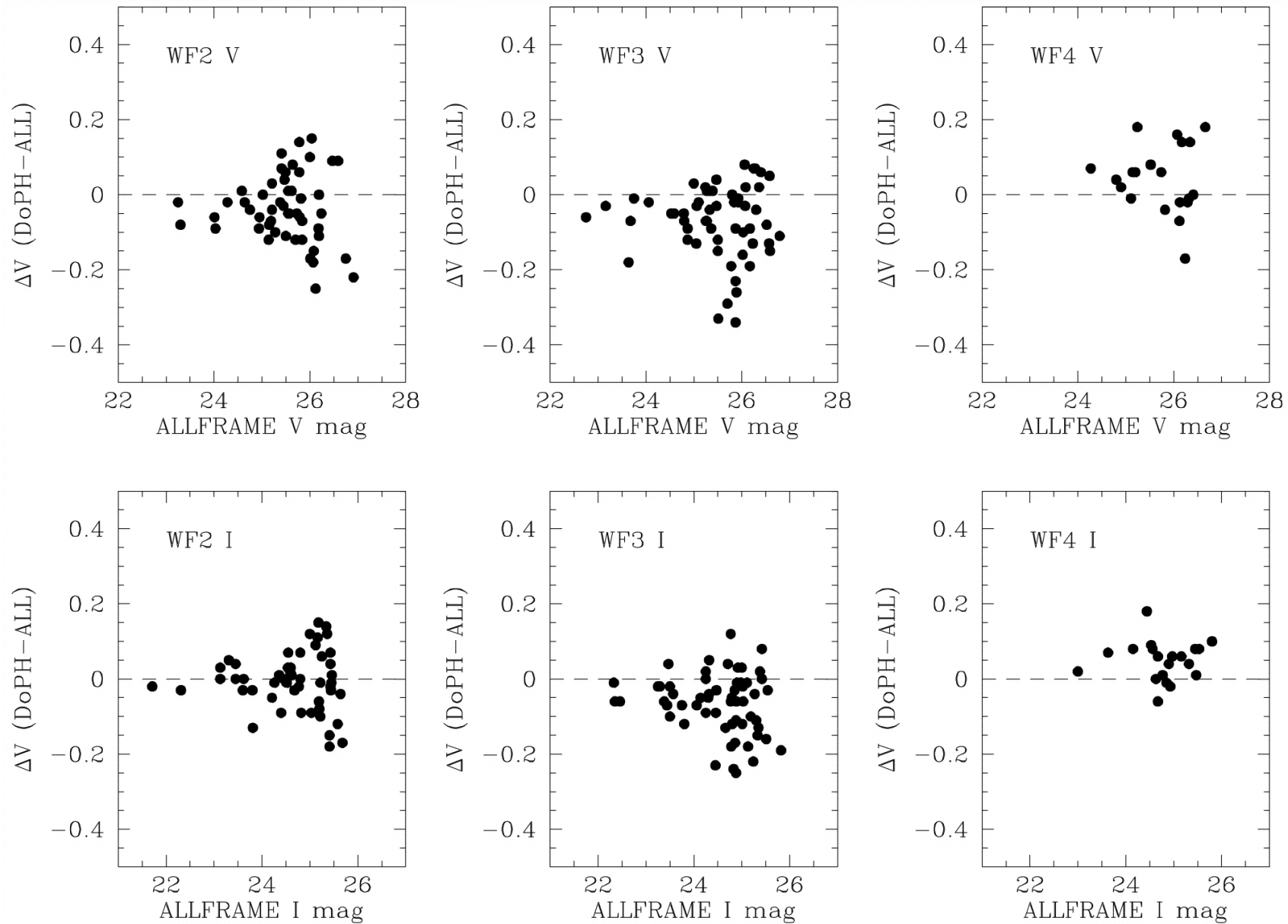
Fig. 2. from The Hubble Space Telescope Key Project on the Extragalactic Distance Scale. XXII. The Discovery of Cepheids in NGC 1326A Prosser et al. 1999 ApJ 525 80 doi:10.1086/307899 https://dx.doi.org/10.1086/307899 © 1999. The American Astronomical Society. All rights reserved. Printed in U.S.A.
