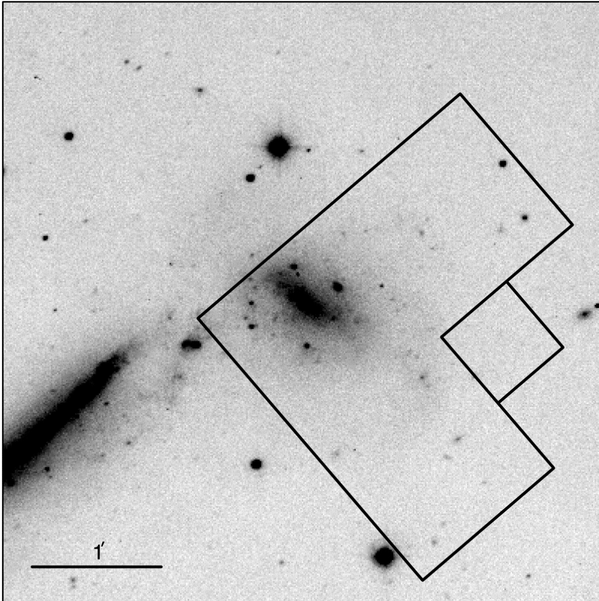
Fig. 1. from The Hubble Space Telescope Key Project on the Extragalactic Distance Scale. XXII. The Discovery of Cepheids in NGC 1326A Prosser et al. 1999 ApJ 525 80 doi:10.1086/307899 https://dx.doi.org/10.1086/307899 © 1999. The American Astronomical Society. All rights reserved. Printed in U.S.A.
