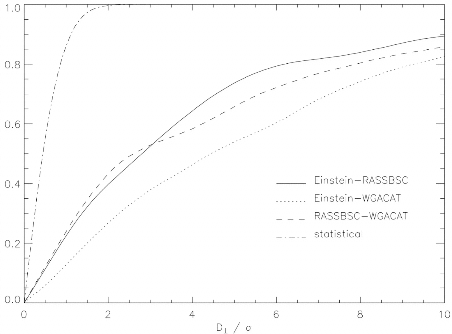
Fig. 4. from On XRay Variability in Active Binary Stars Kashyap & Drake 1999 ApJ 524 988 doi:10.1086/307821 https://dx.doi.org/10.1086/307821 © 1999. The American Astronomical Society. All rights reserved. Printed in U.S.A.
